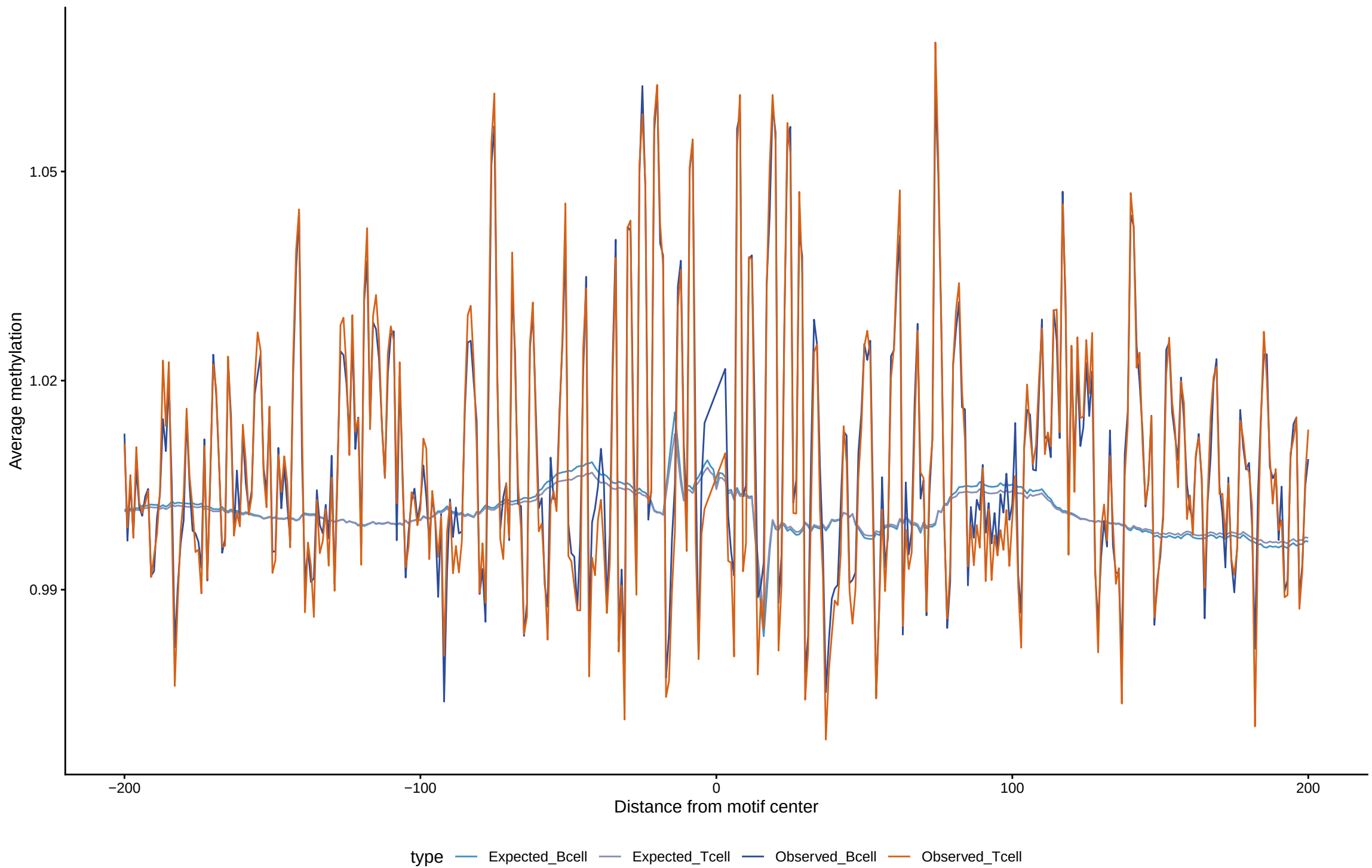
Expected vs observed footprints for PITX1
