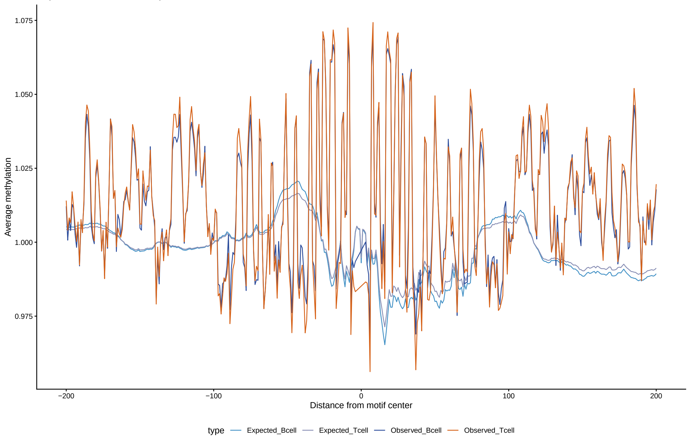
Expected vs observed footprints for PITX2
