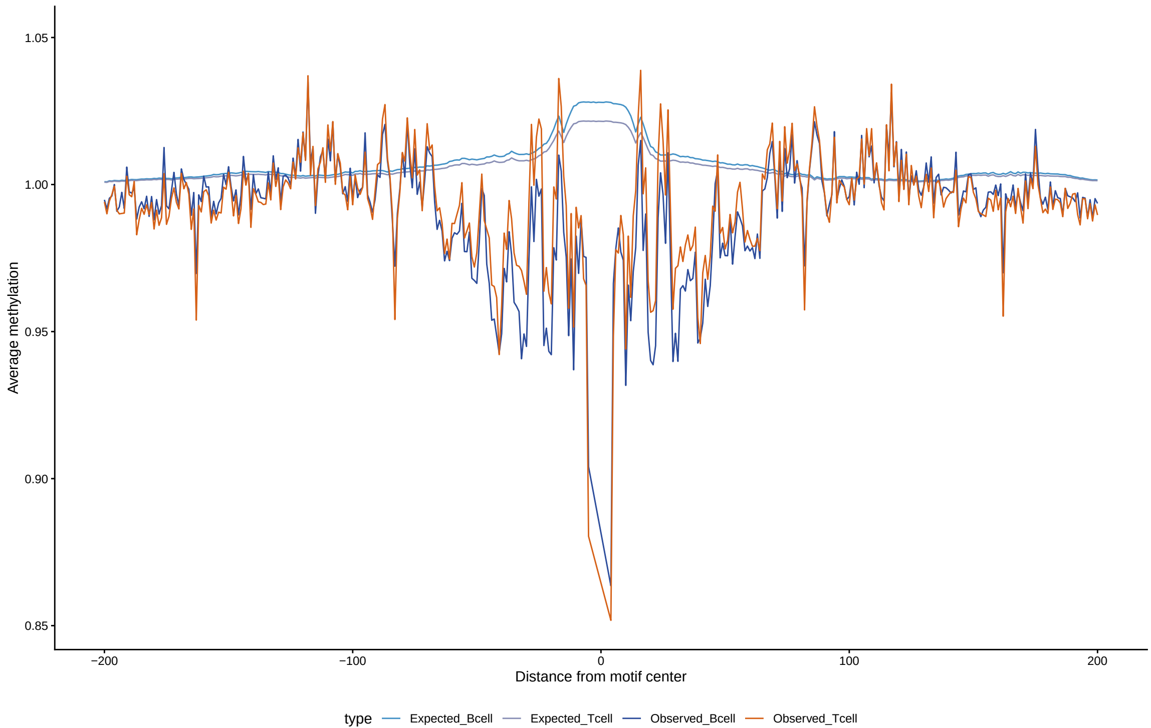
Expected vs observed footprints for POU2F3
