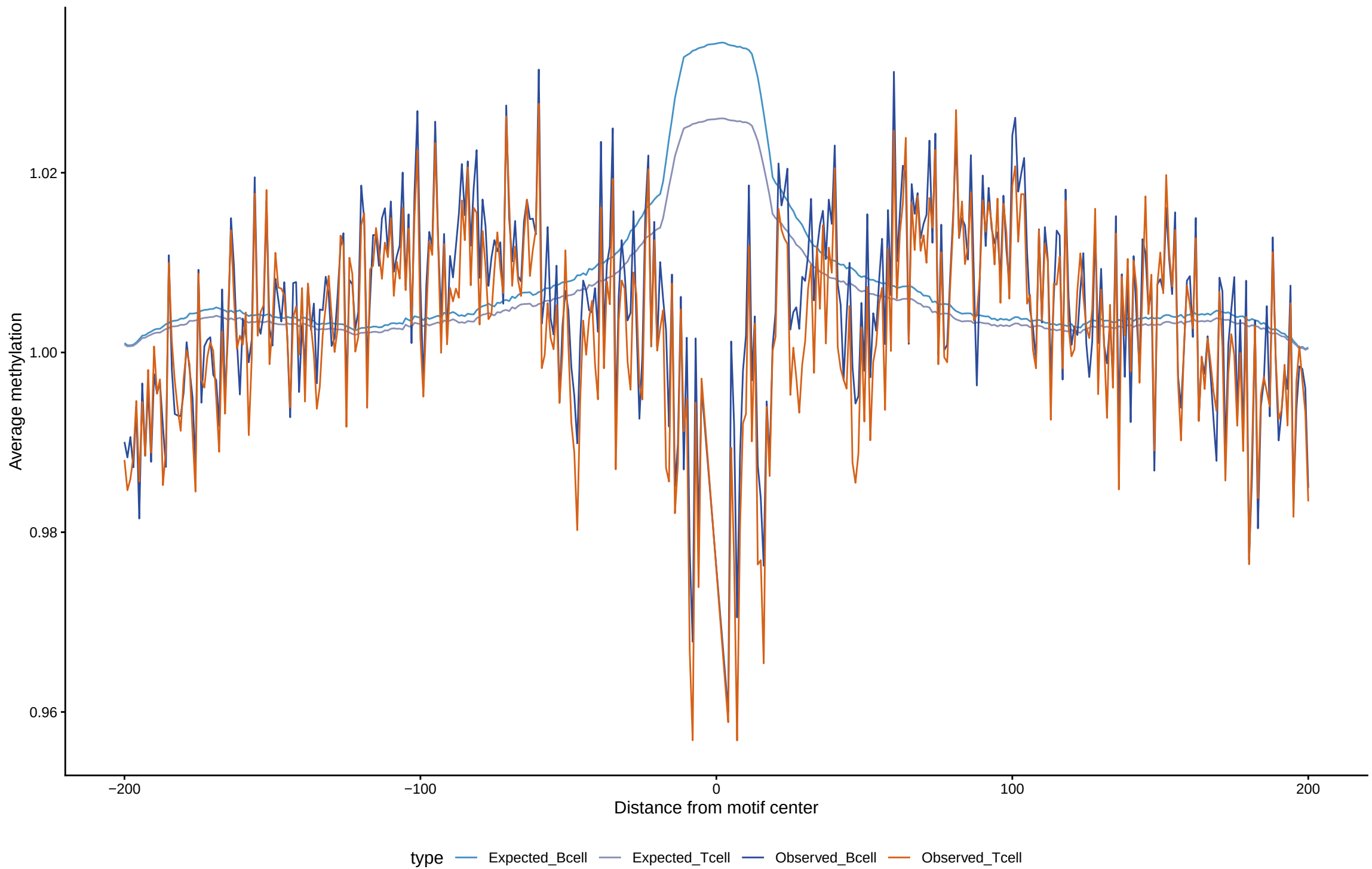
Expected vs observed footprints for PRRX1
