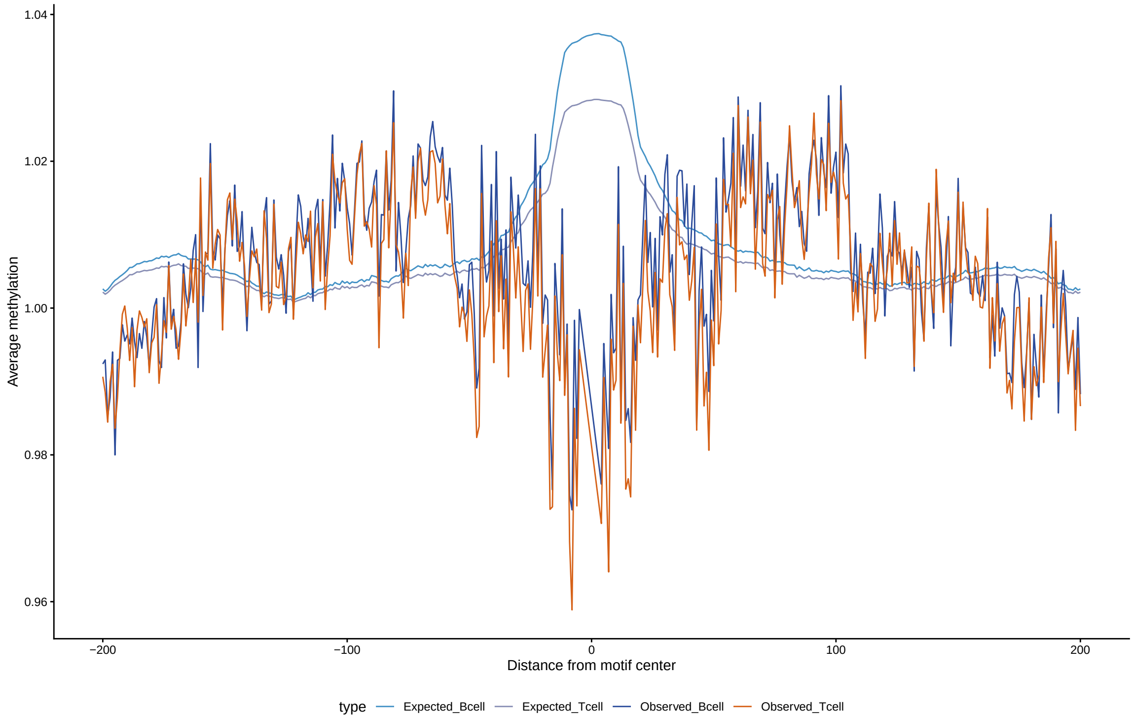
Expected vs observed footprints for RAX
