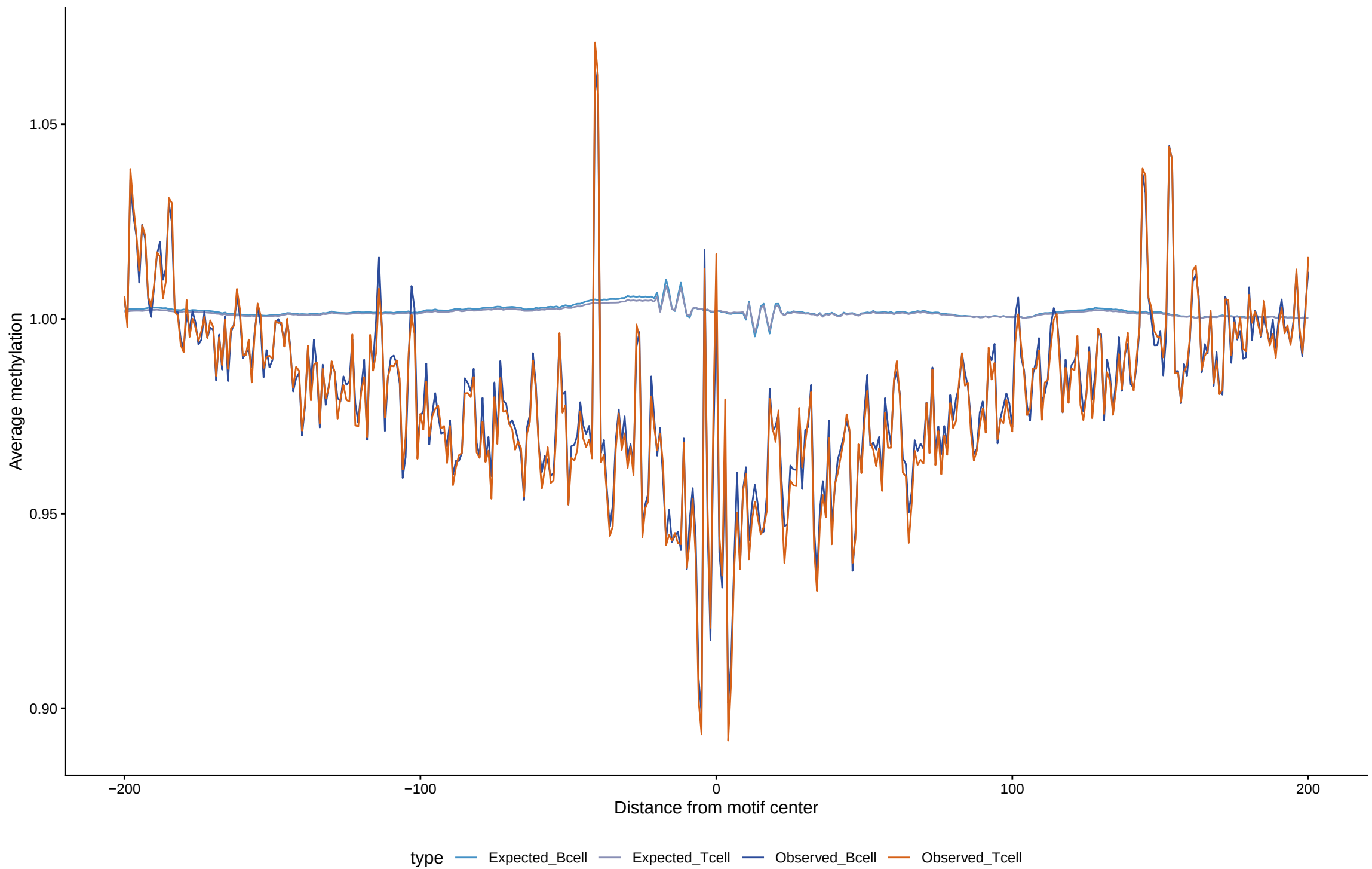
Expected vs observed footprints for RFX3
