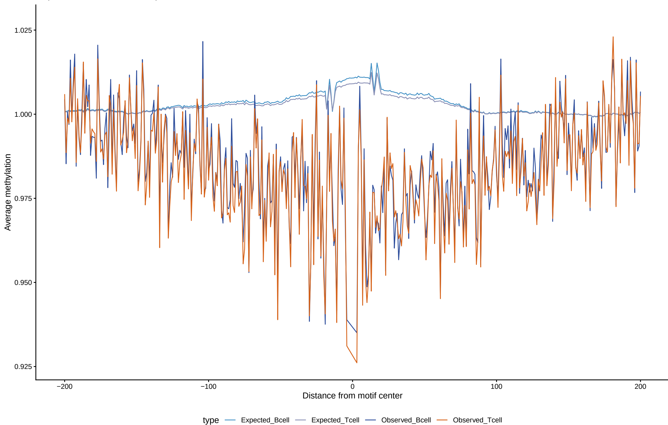
Expected vs observed footprints for RFX7
