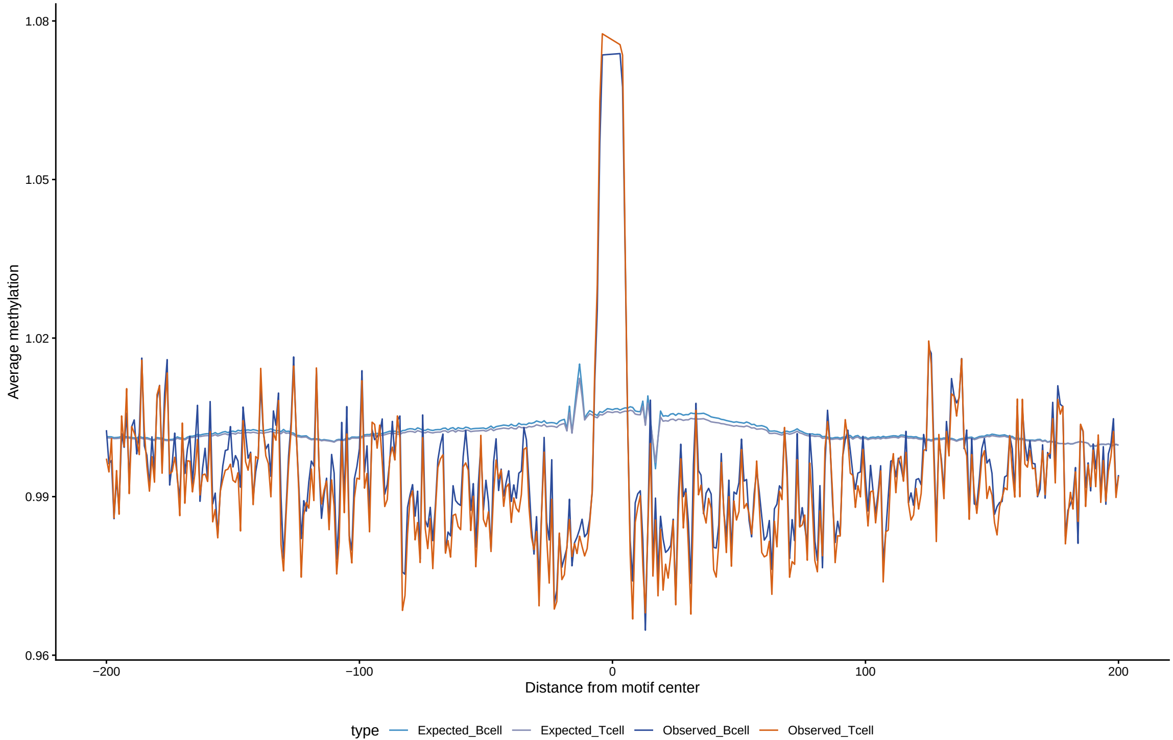
Expected vs observed footprints for SOX18
