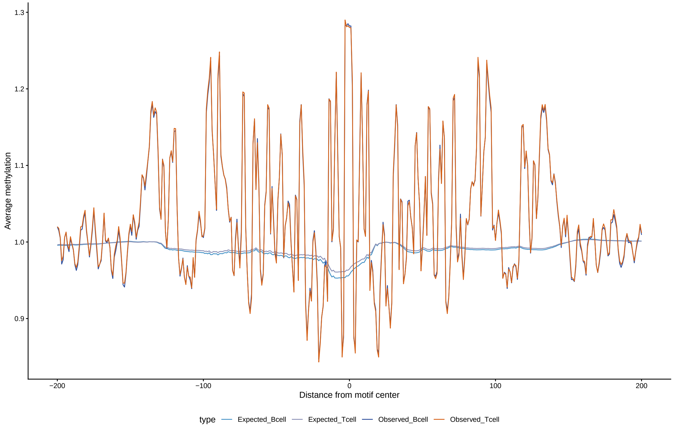
Expected vs observed footprints for SP9
