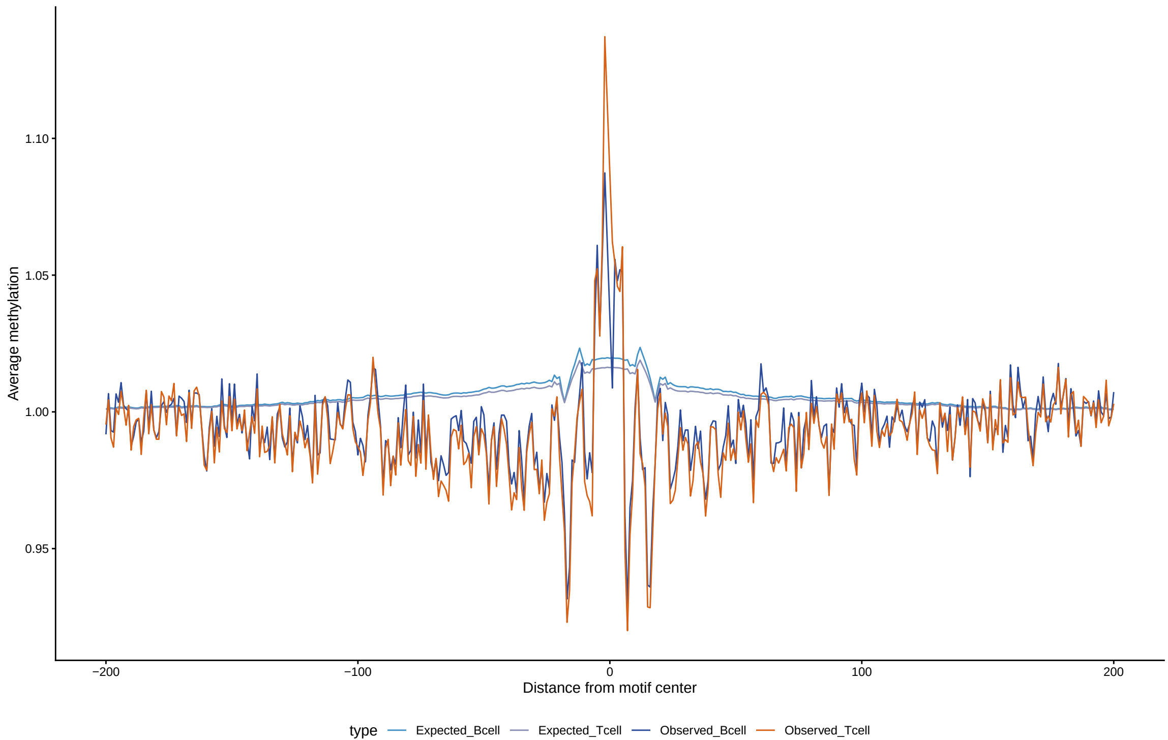
Expected vs observed footprints for SRF
