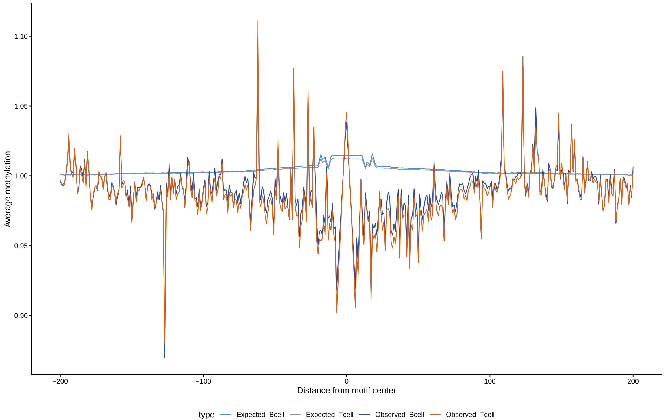
Expected vs observed footprints for STAT1
