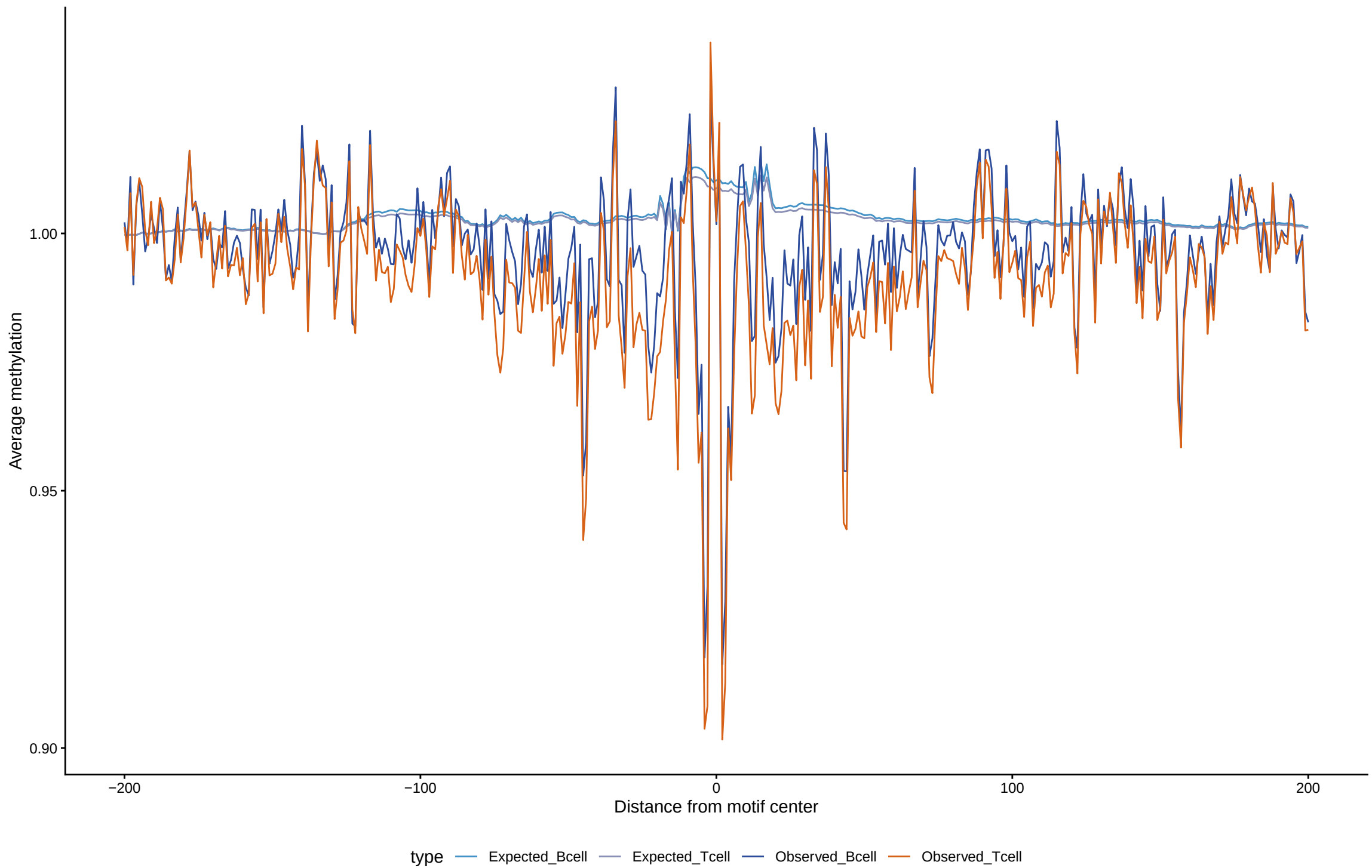
Expected vs observed footprints for TBR1
