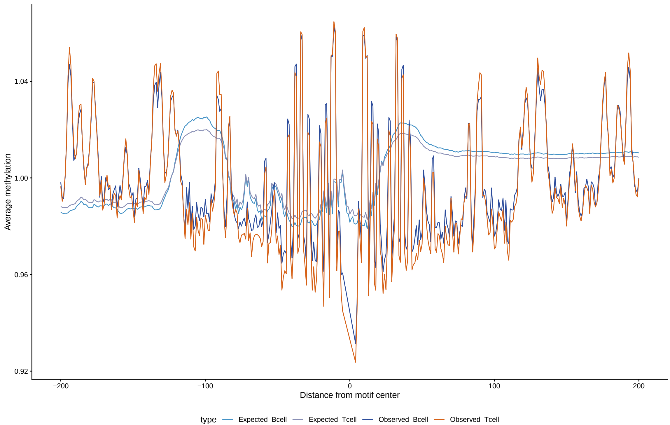
Expected vs observed footprints for TBX1
