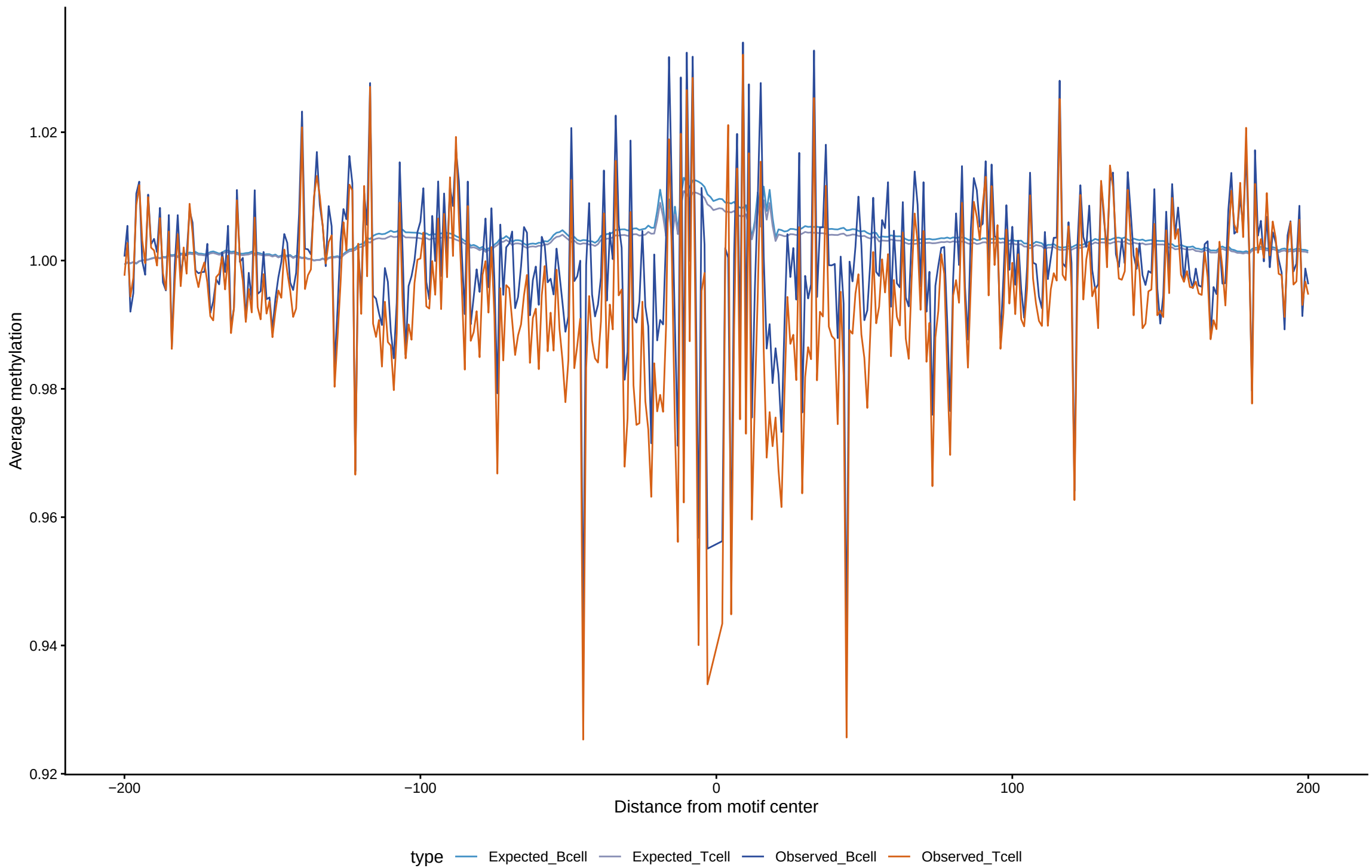
Expected vs observed footprints for TBX20
