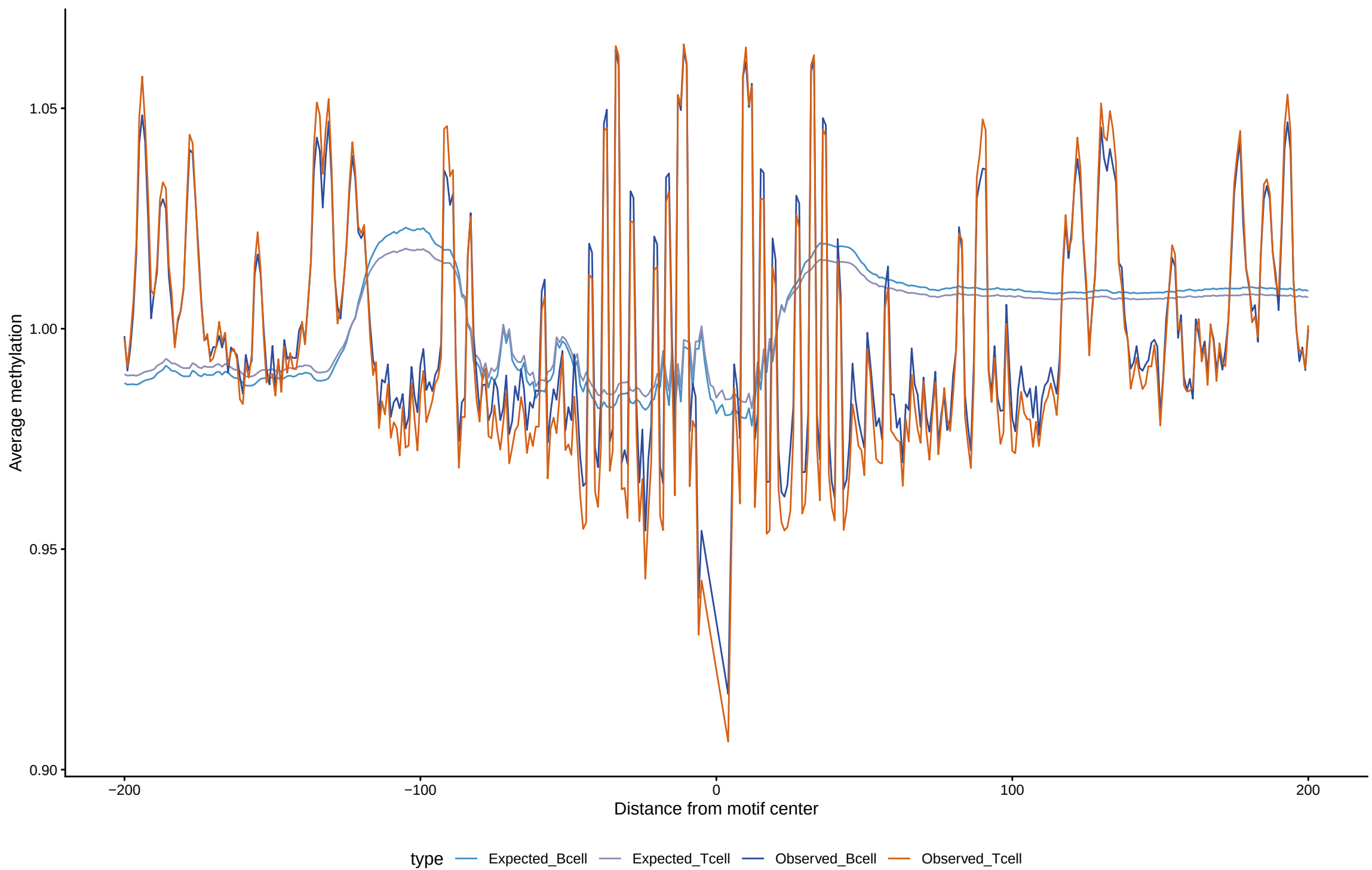
Expected vs observed footprints for TBX4
