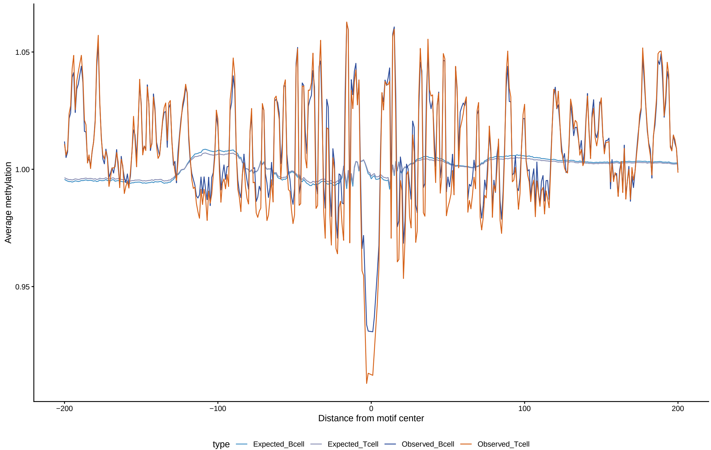
Expected vs observed footprints for TBX6
