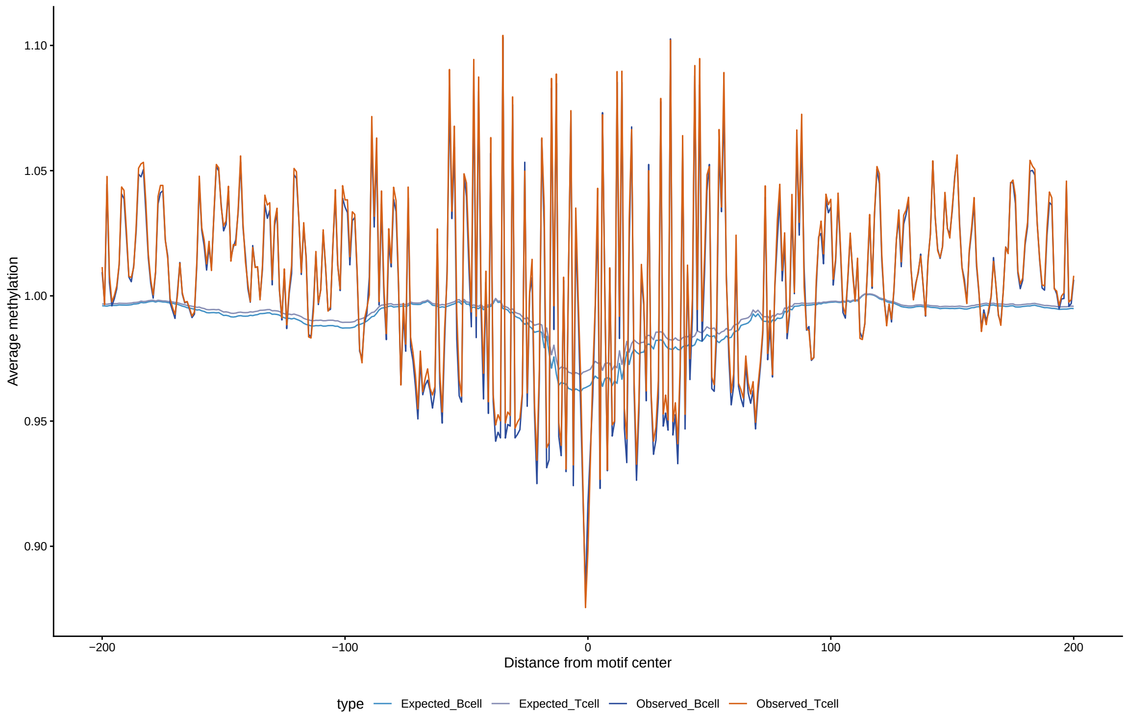
Expected vs observed footprints for TCF12(var.2)
