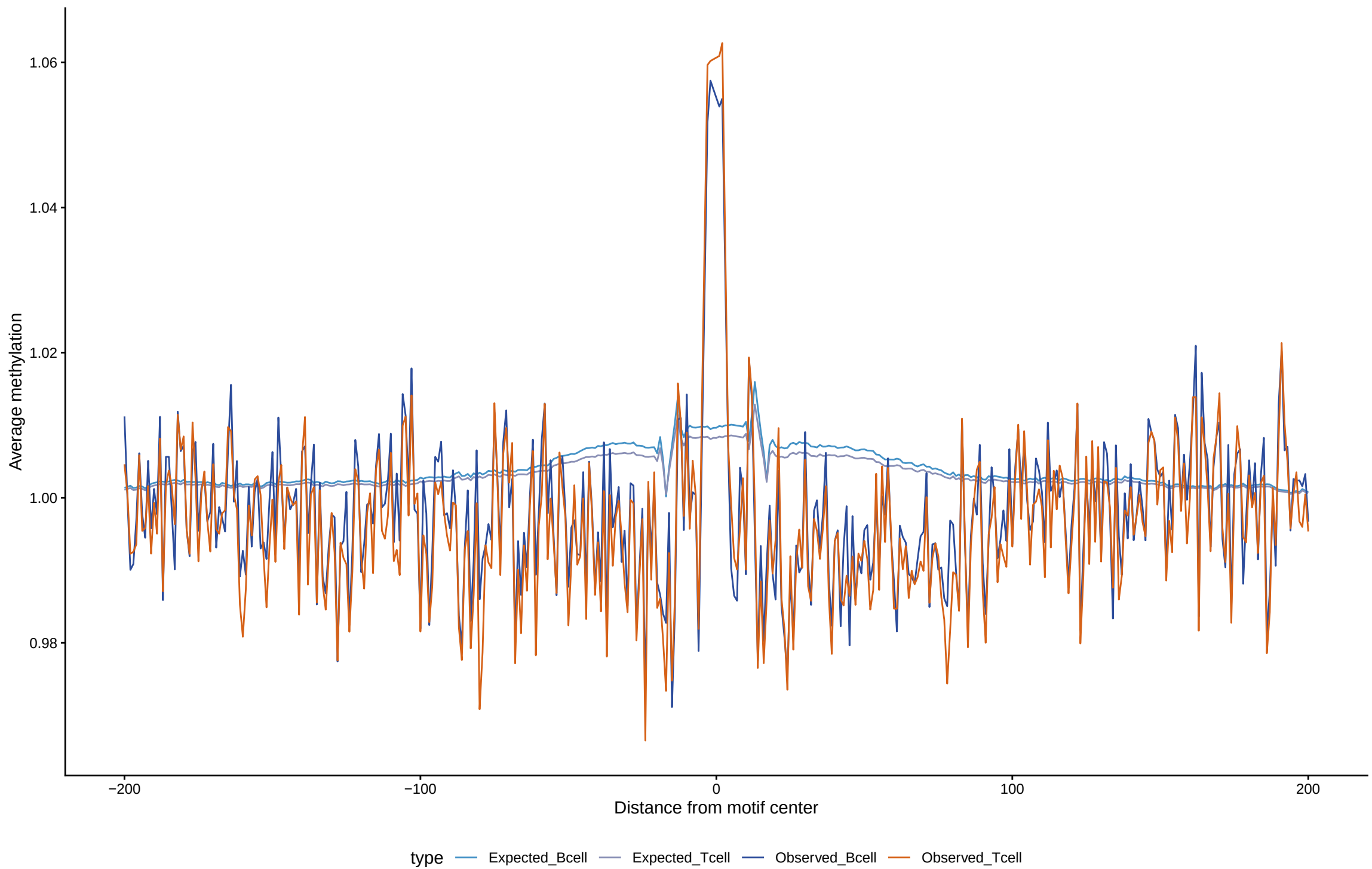
Expected vs observed footprints for TCF21(var.2)
