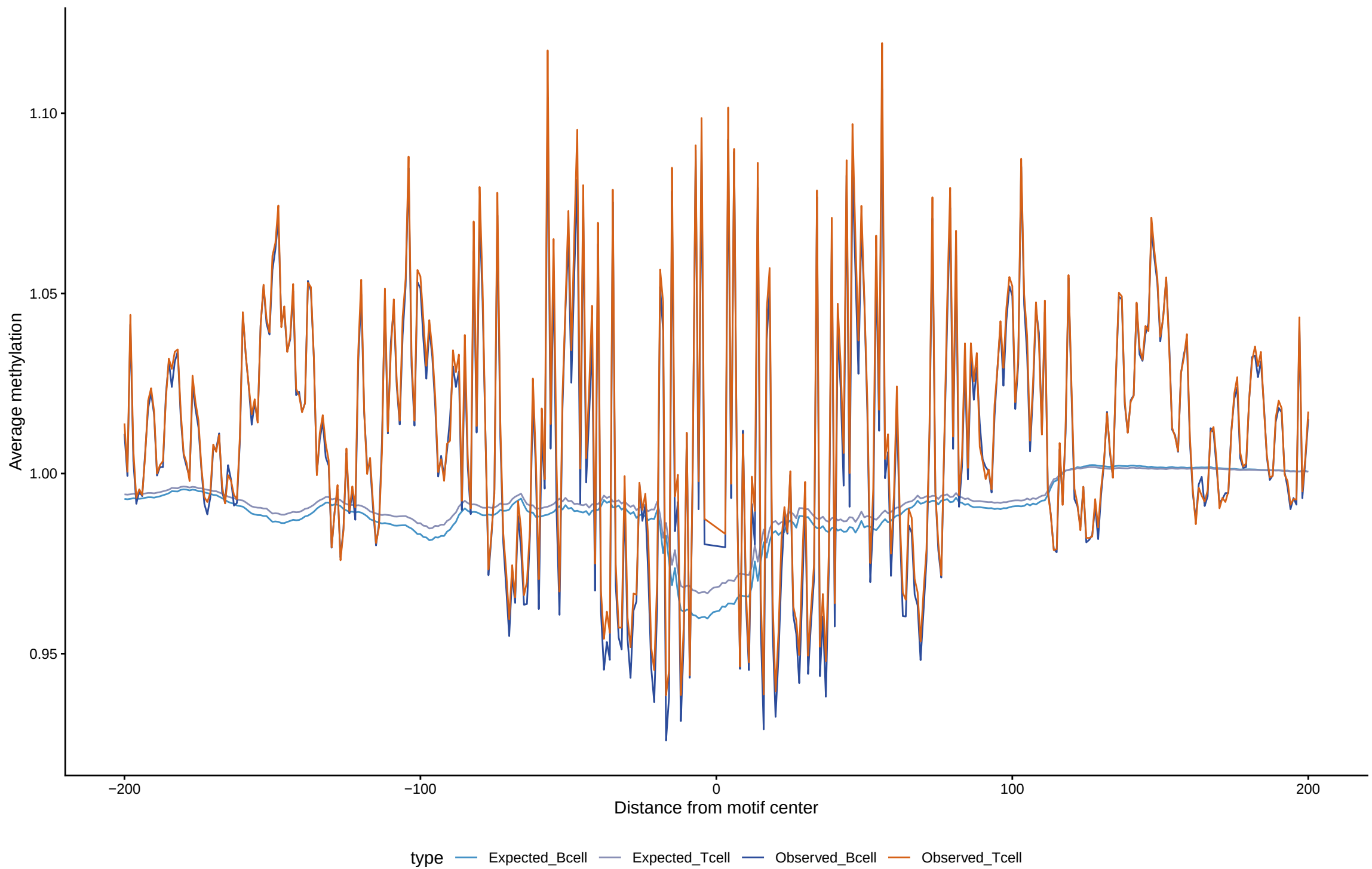
Expected vs observed footprints for TCF4
