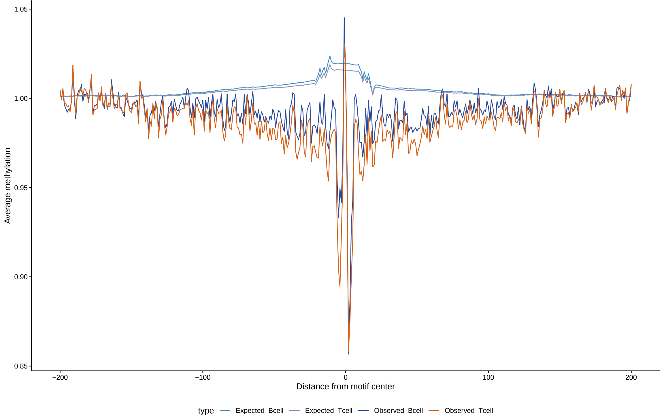
Expected vs observed footprints for TCF7L1
