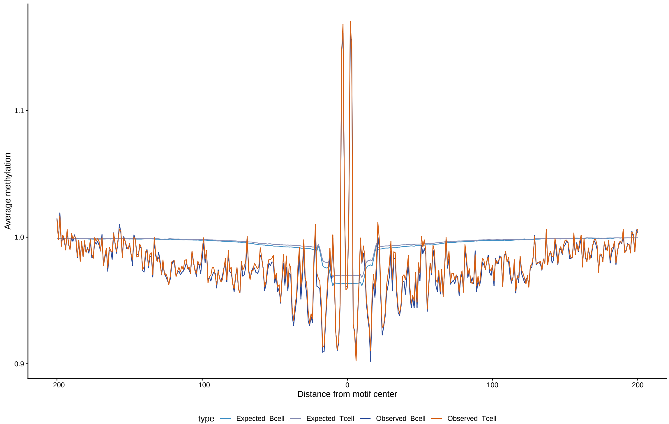
Expected vs observed footprints for TFAP2A(var.2)
