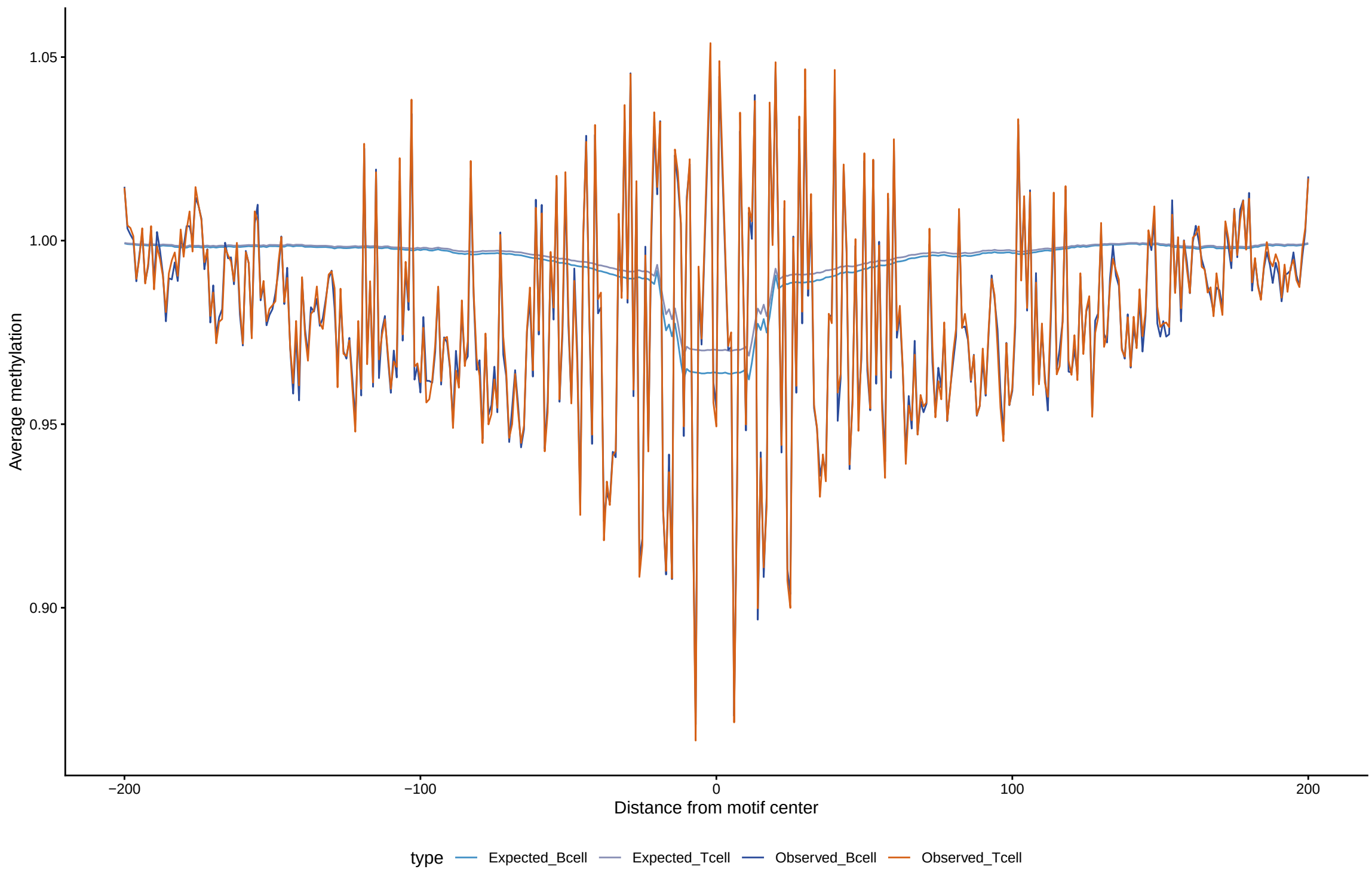
Expected vs observed footprints for TFAP2B(var.2)
