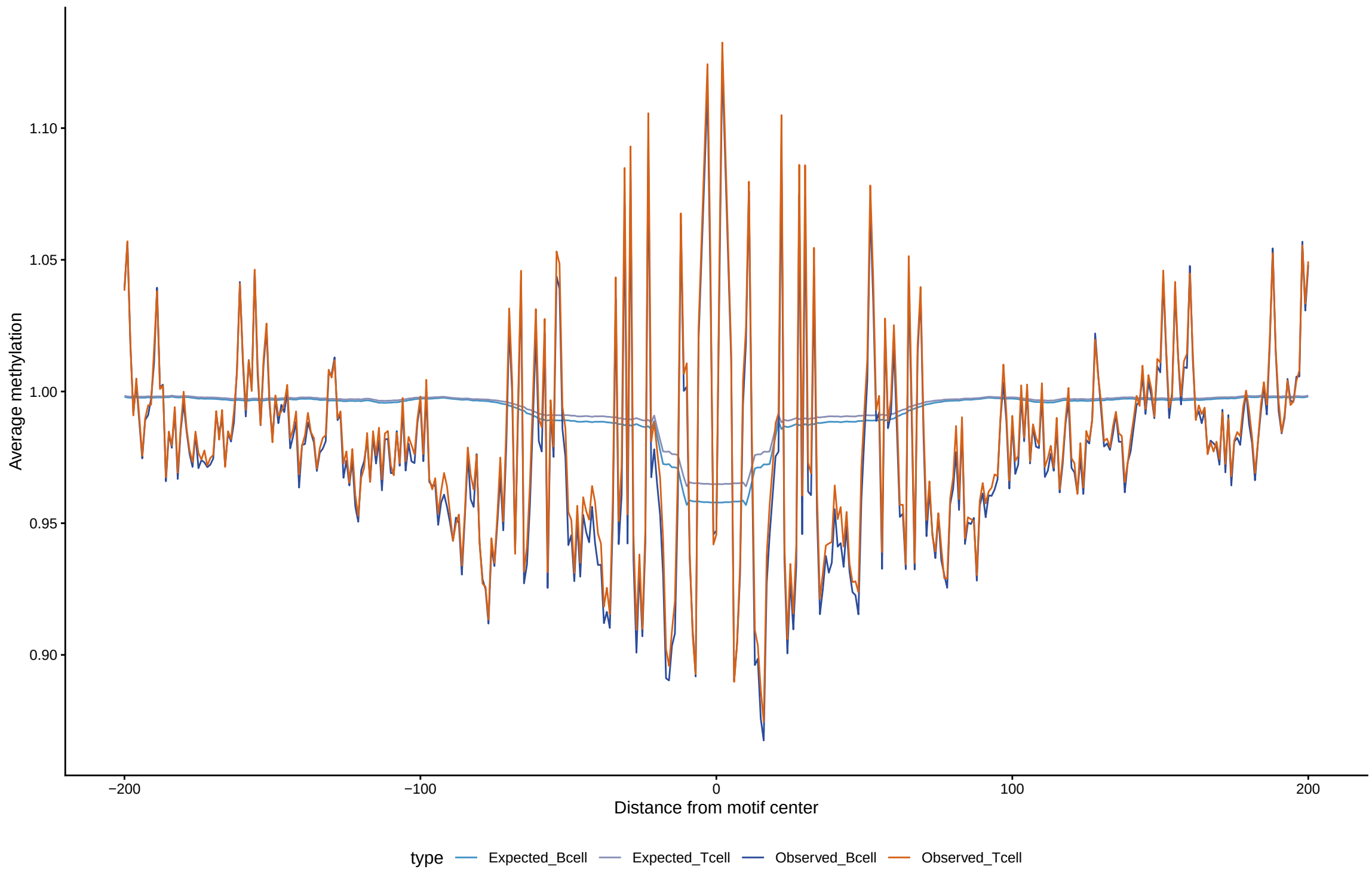
Expected vs observed footprints for TFAP2C(var.3)
