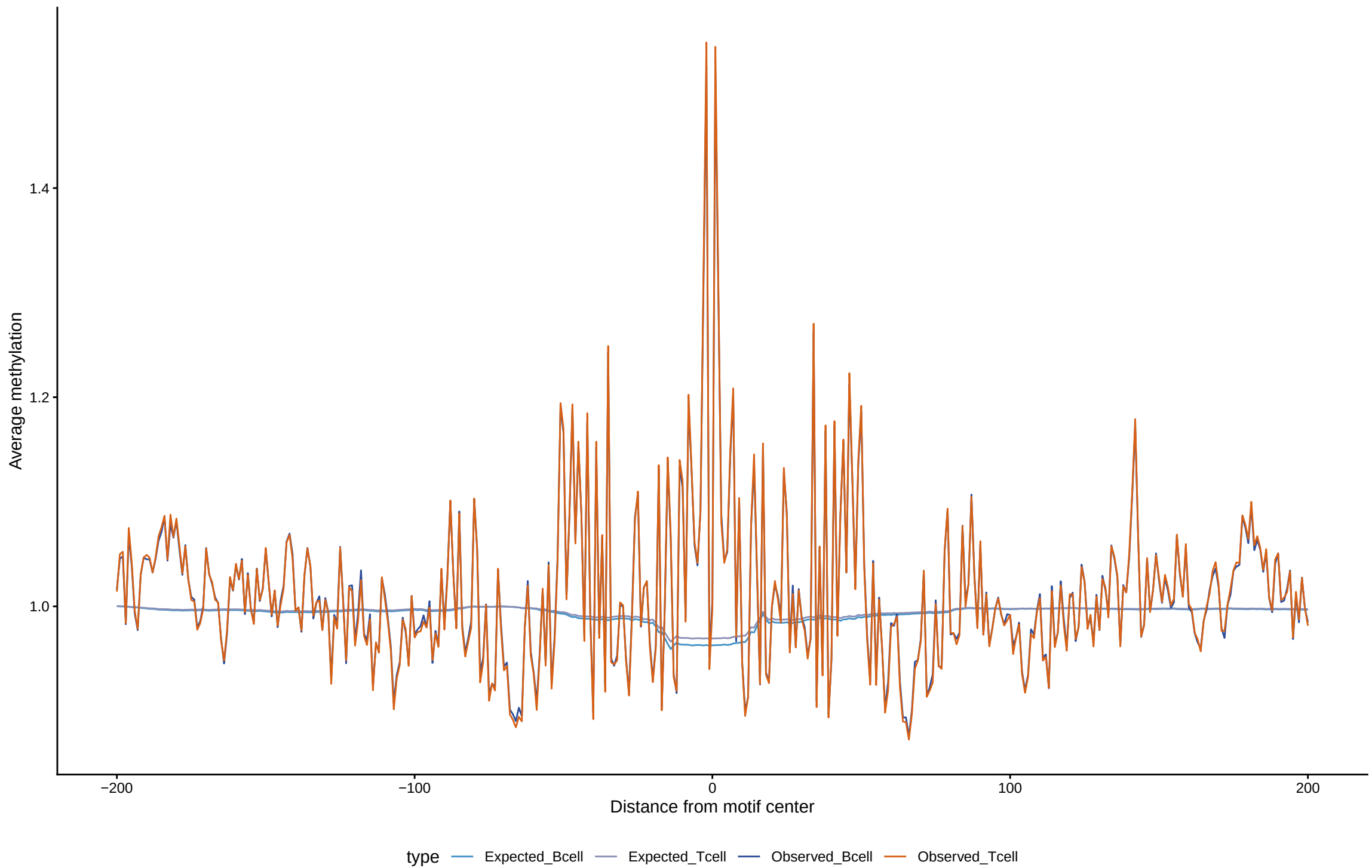
Expected vs observed footprints for TFDP1
