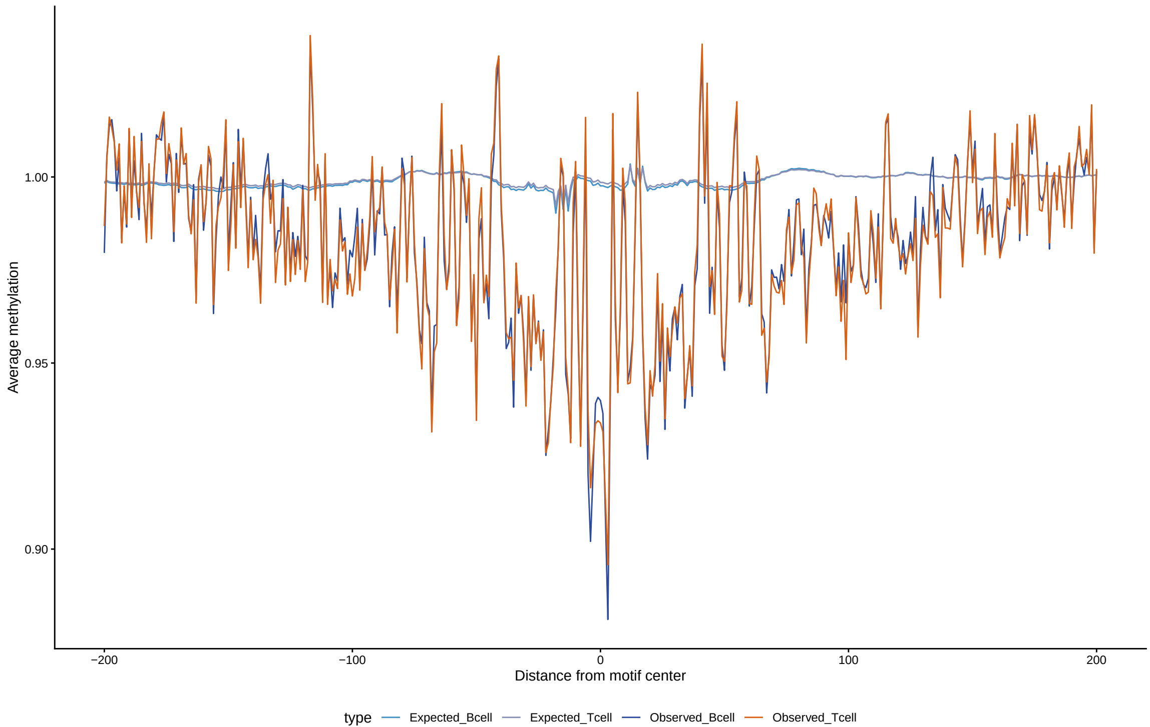
Expected vs observed footprints for TFE3
