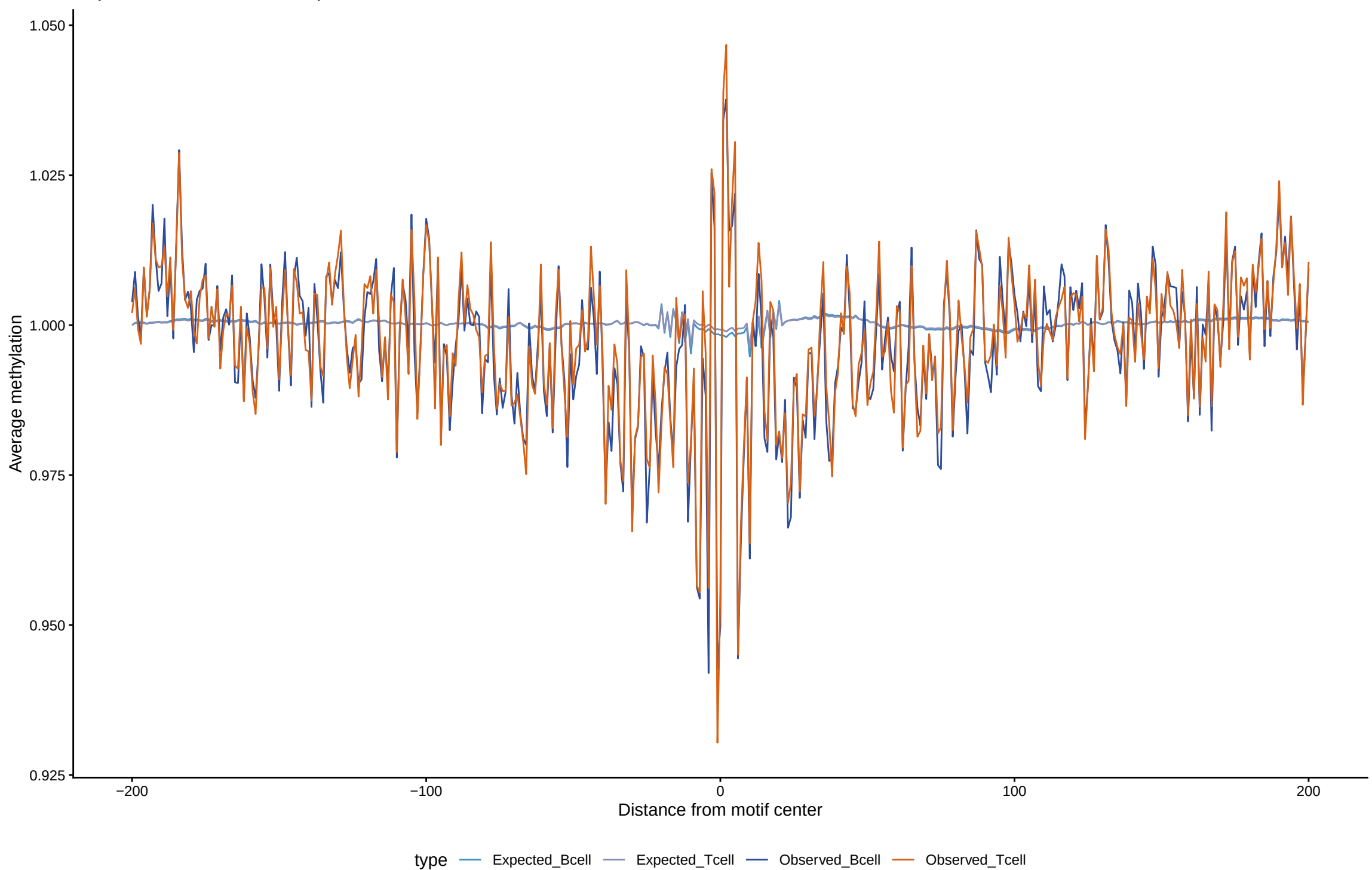
Expected vs observed footprints for TGIF2
