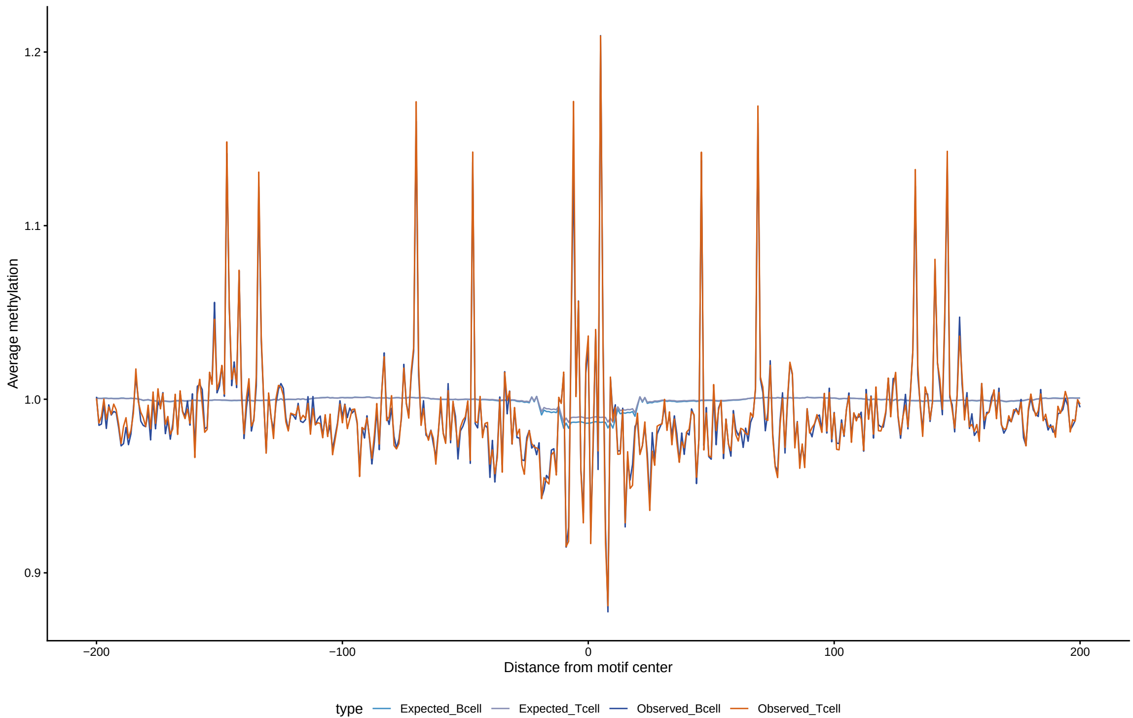
Expected vs observed footprints for THRB(var.2)
