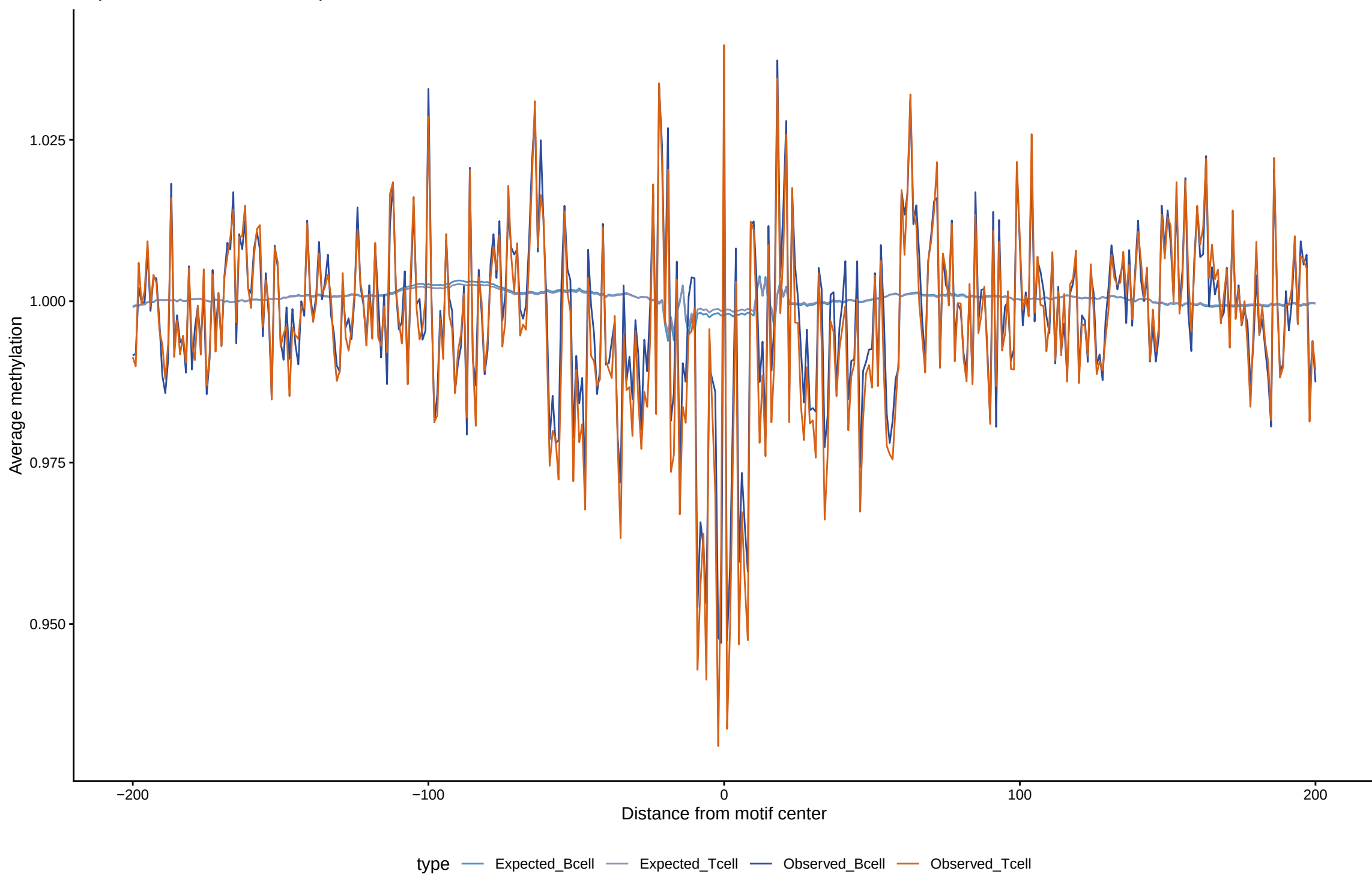
Expected vs observed footprints for THRB
