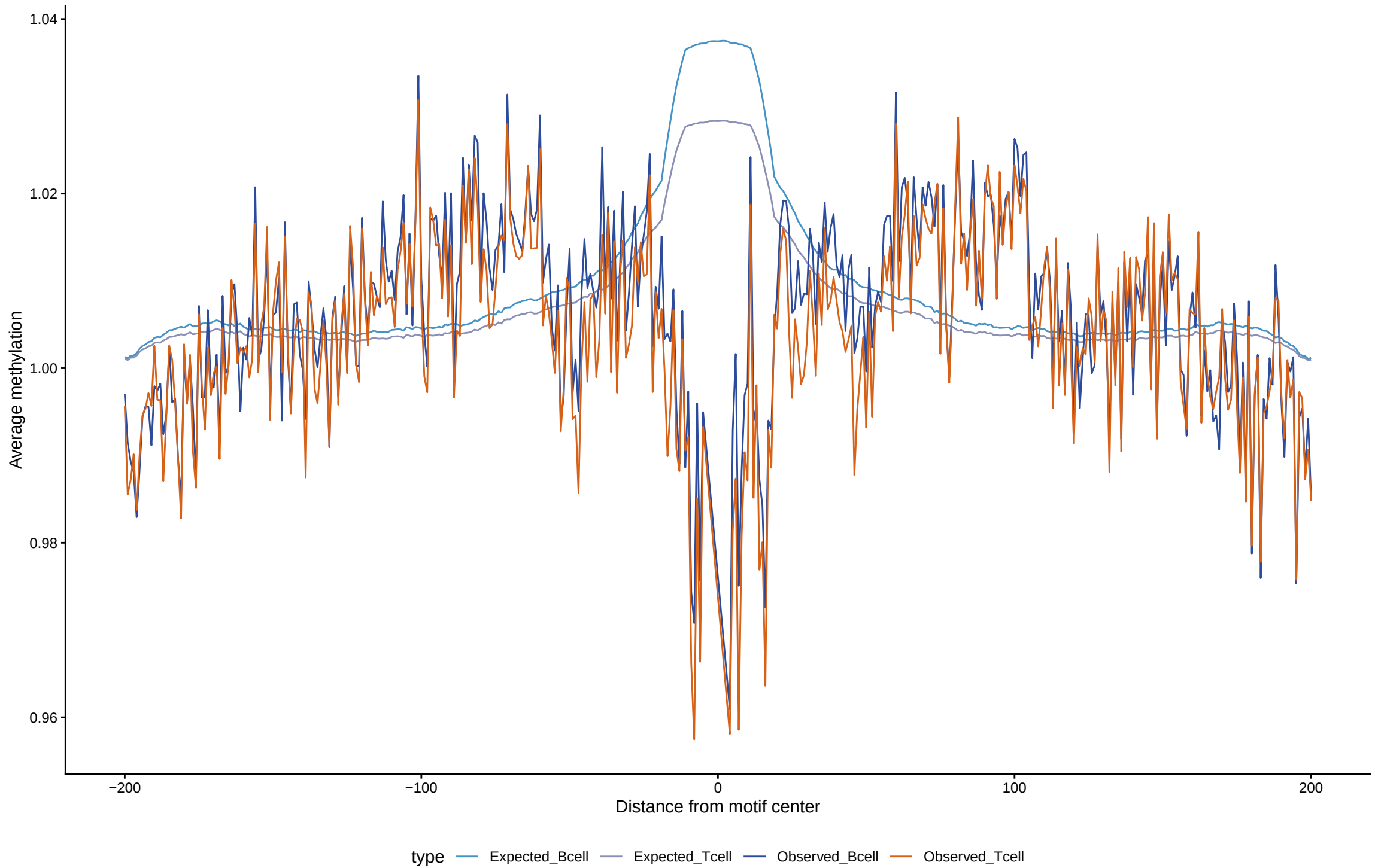
Expected vs observed footprints for UNCX
