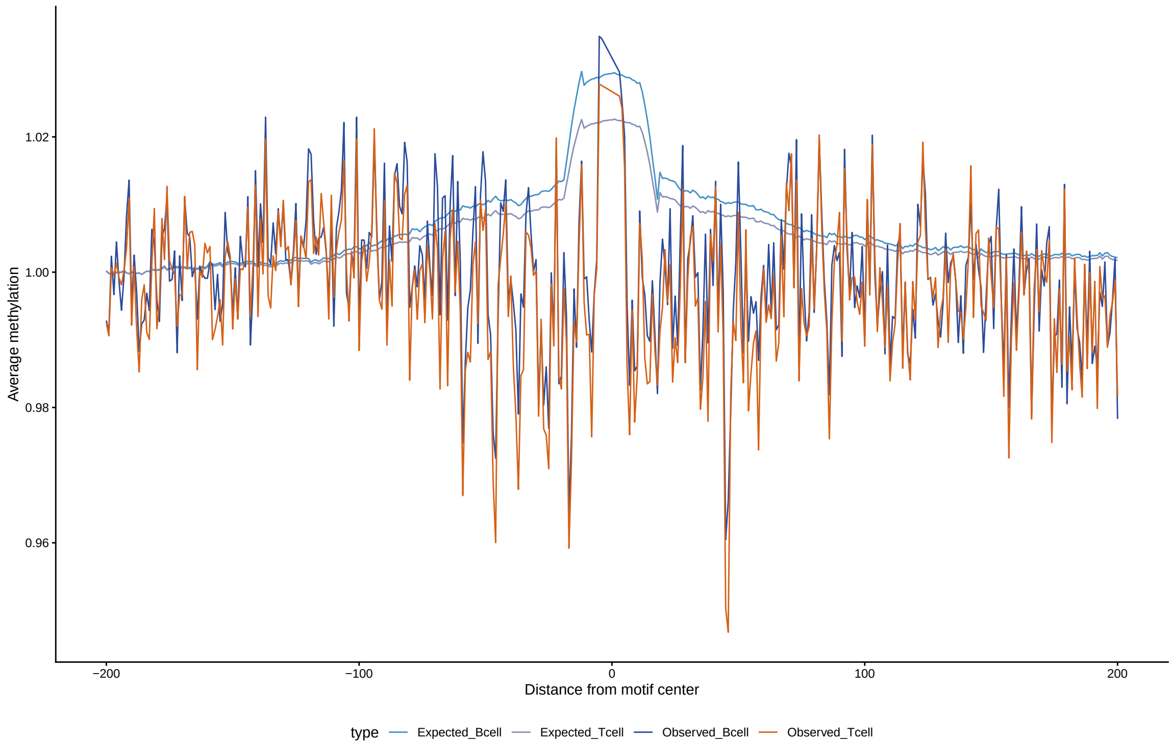
Expected vs observed footprints for VAX2
