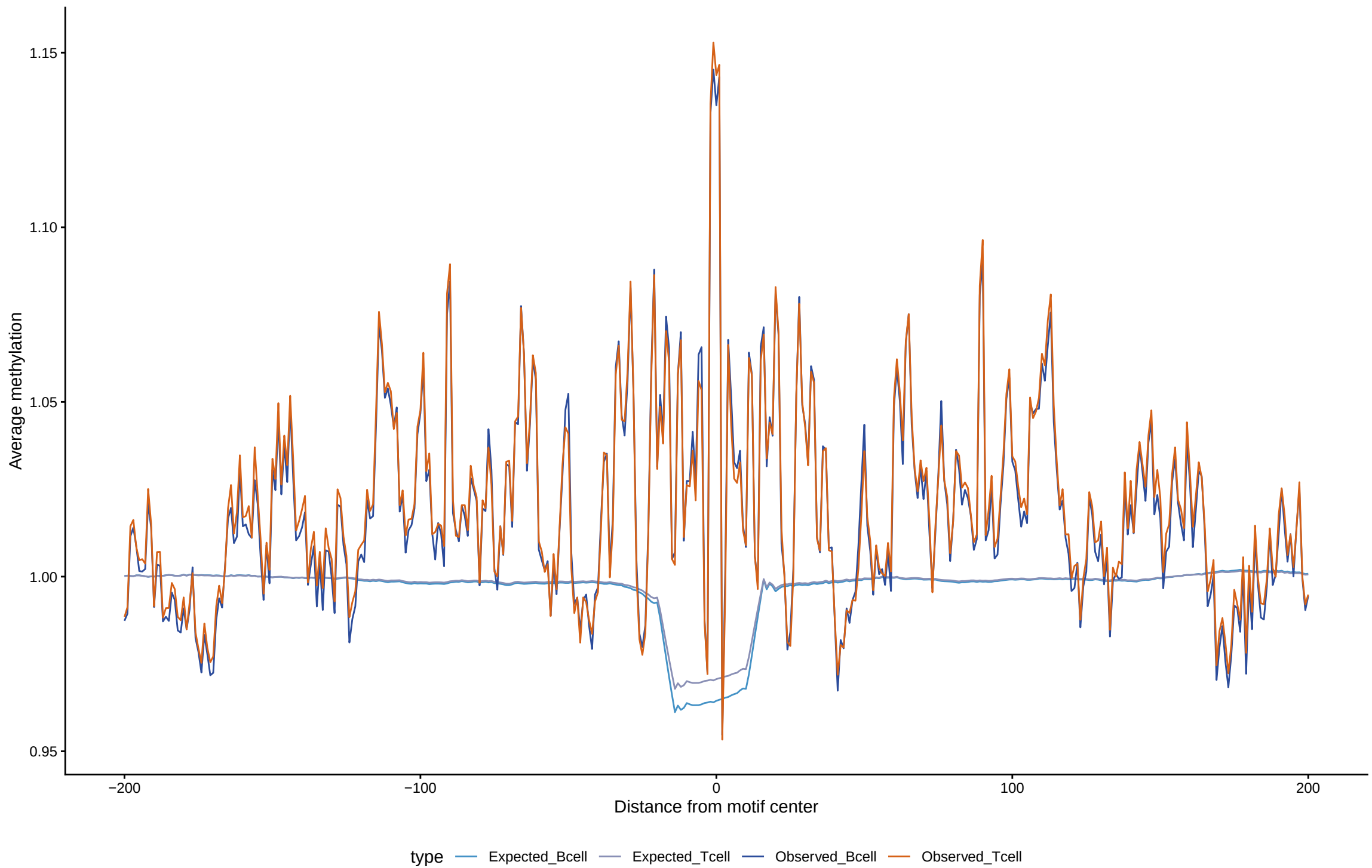
Expected vs observed footprints for VEZF1
