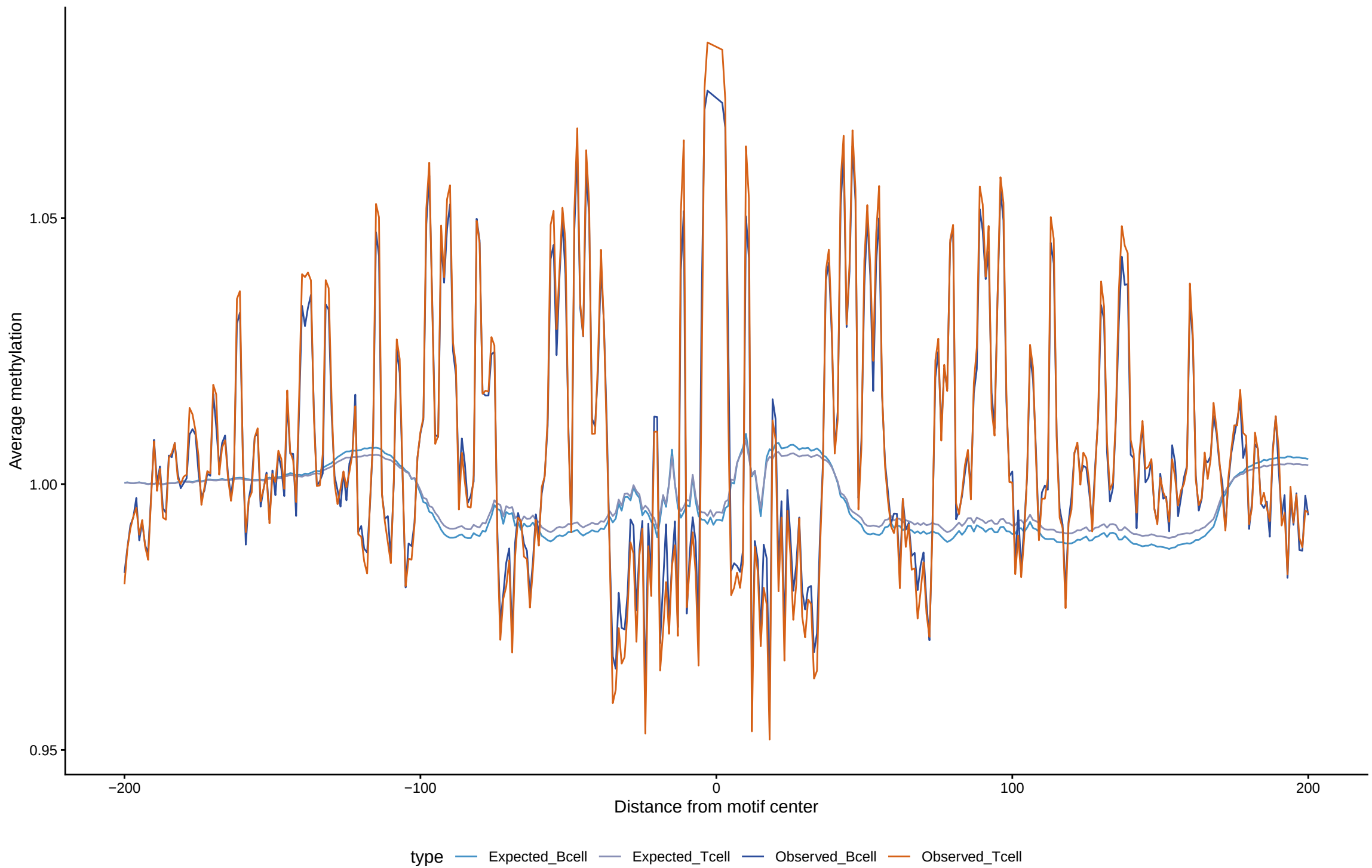
Expected vs observed footprints for YY1
