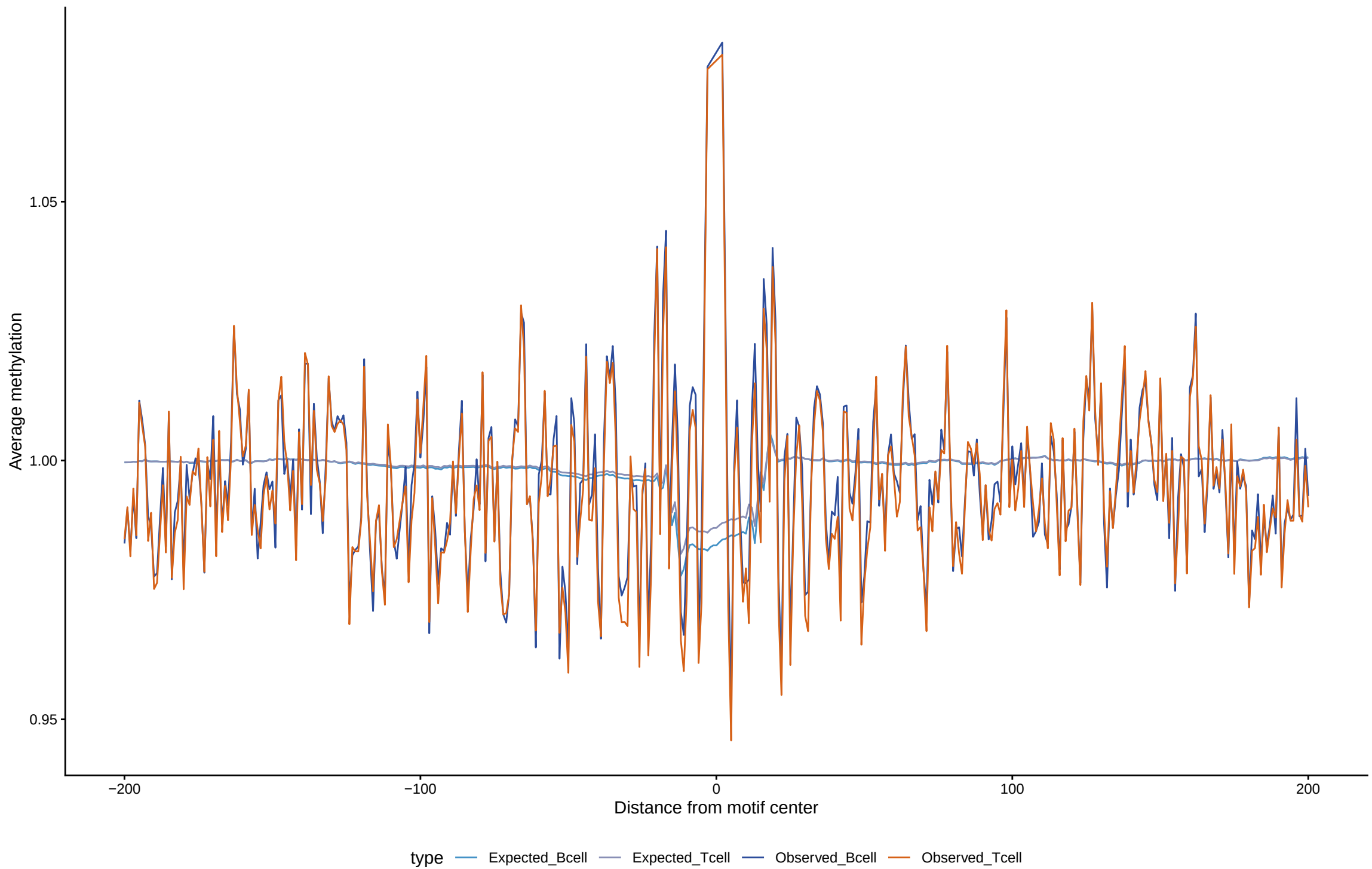
Expected vs observed footprints for ZBTB7B
