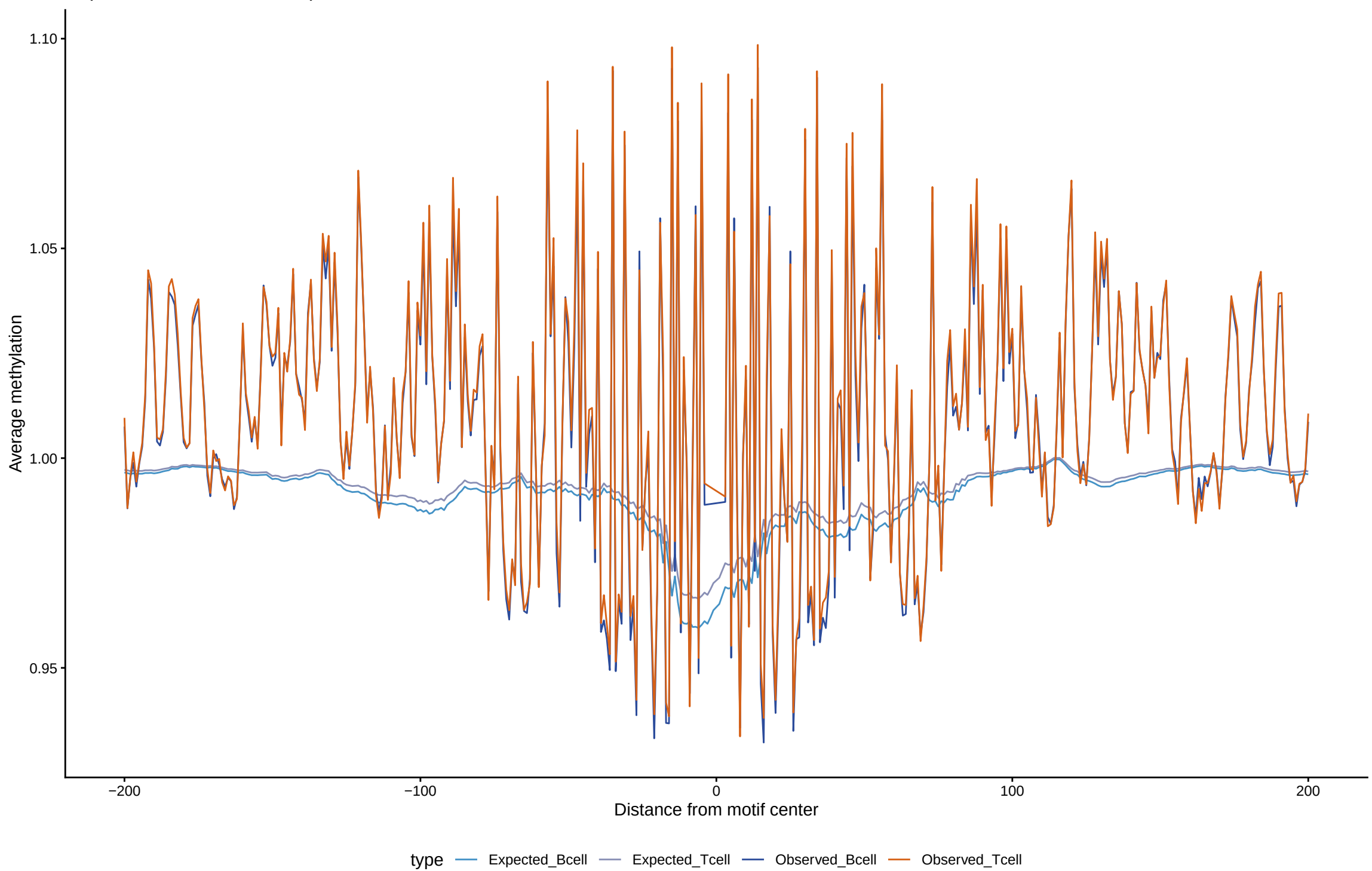
Expected vs observed footprints for ZEB1
