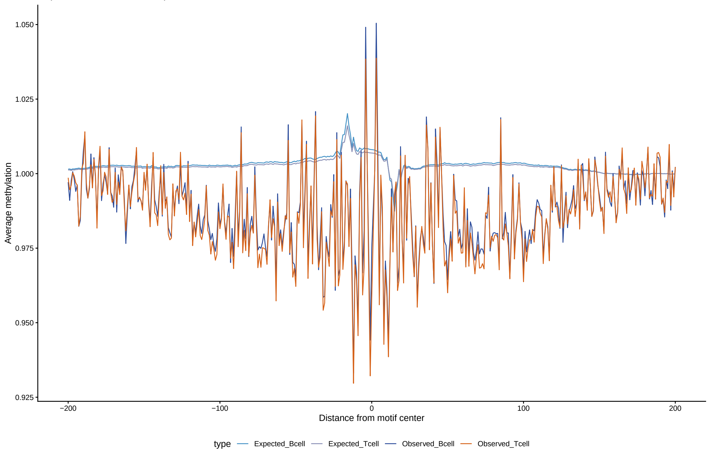
Expected vs observed footprints for ZFP42
