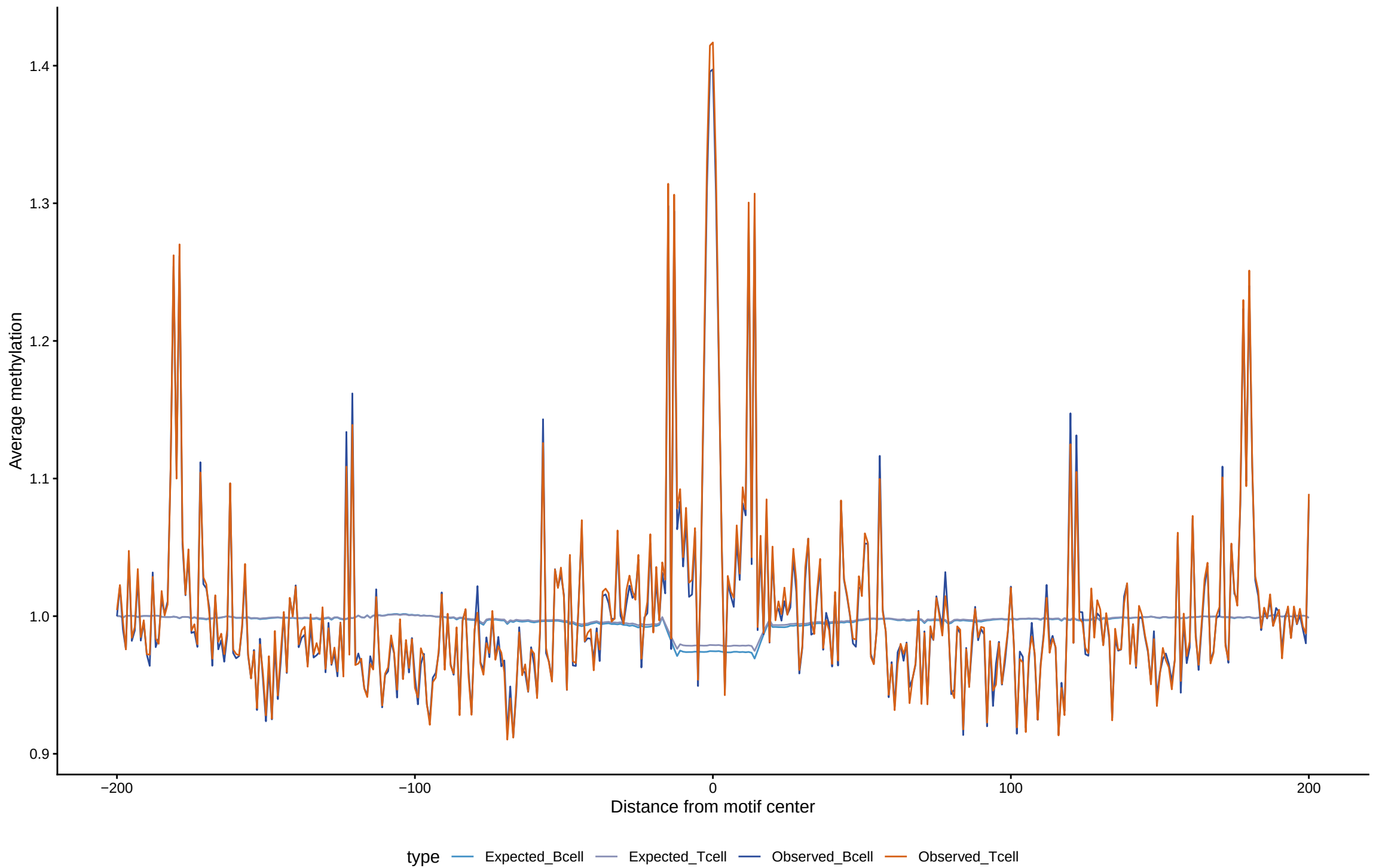
Expected vs observed footprints for ZFP57
