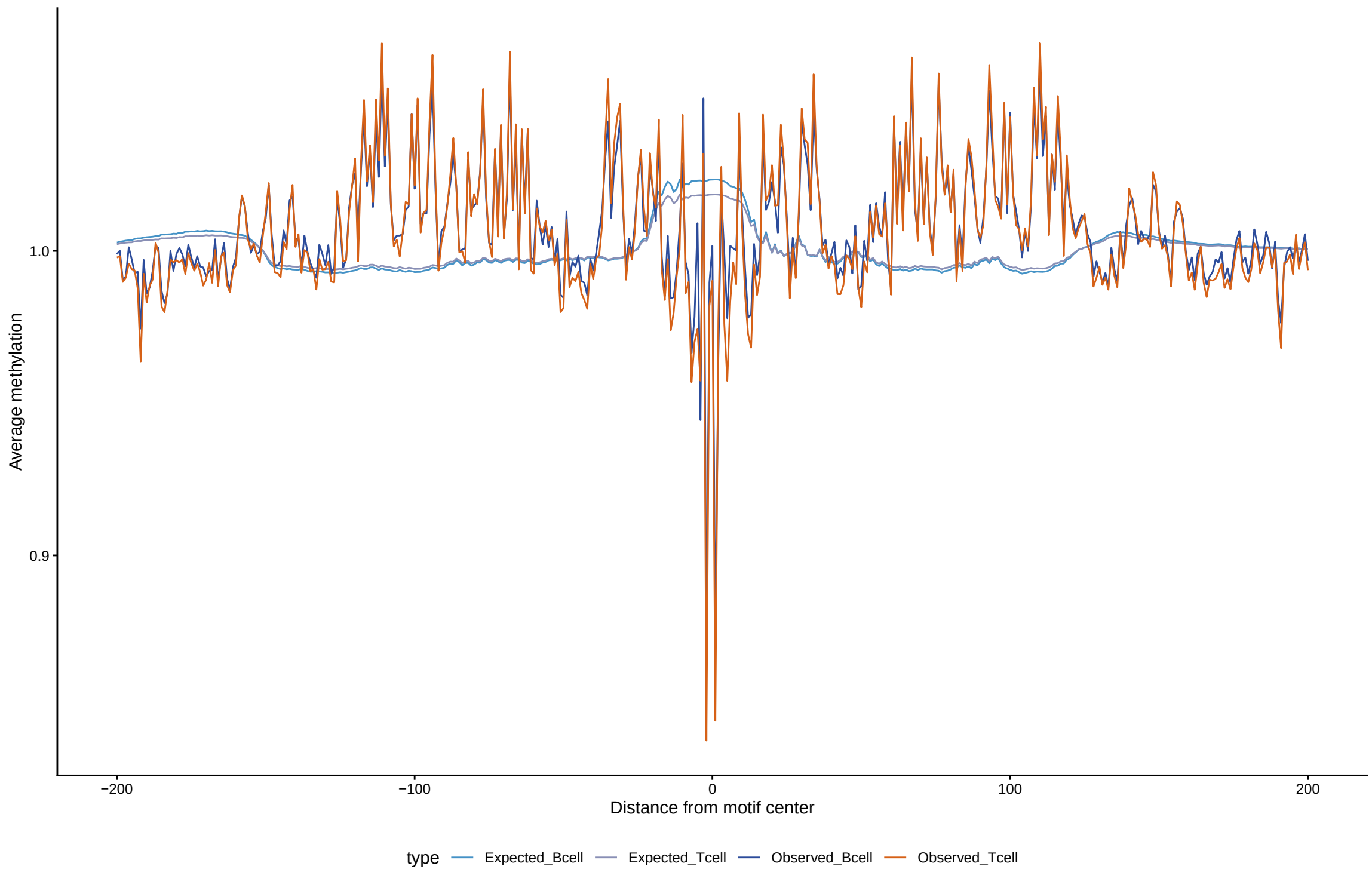
Expected vs observed footprints for ZNF136
