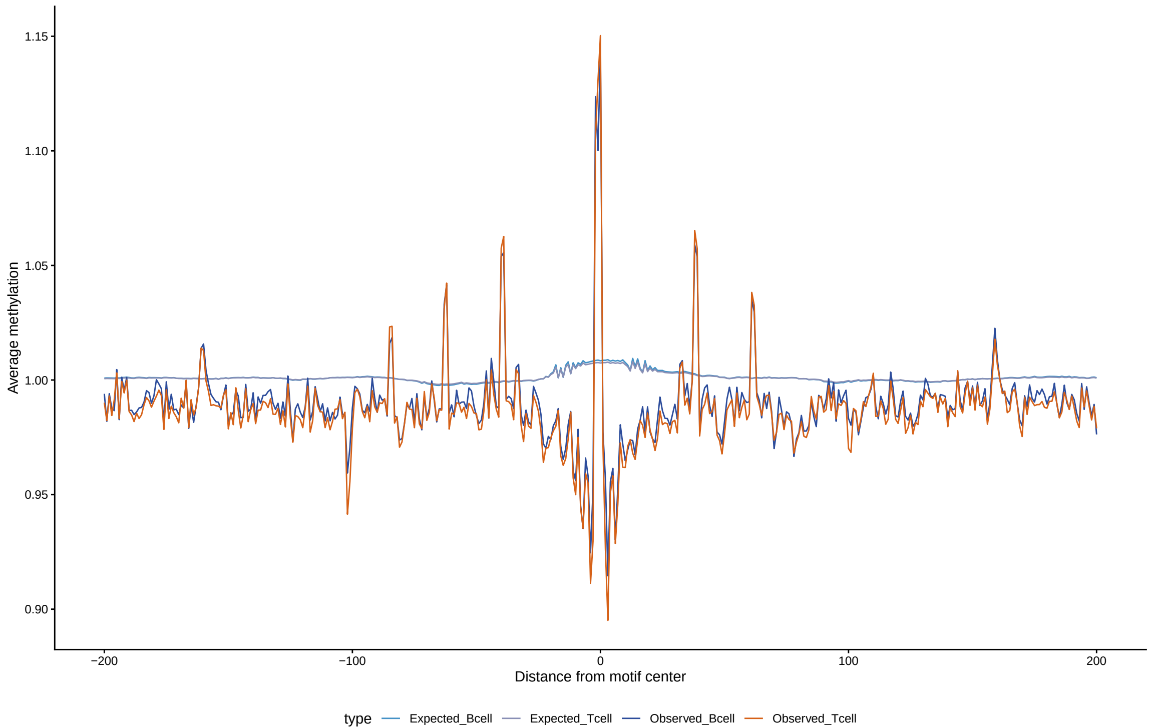
Expected vs observed footprints for ZNF274
