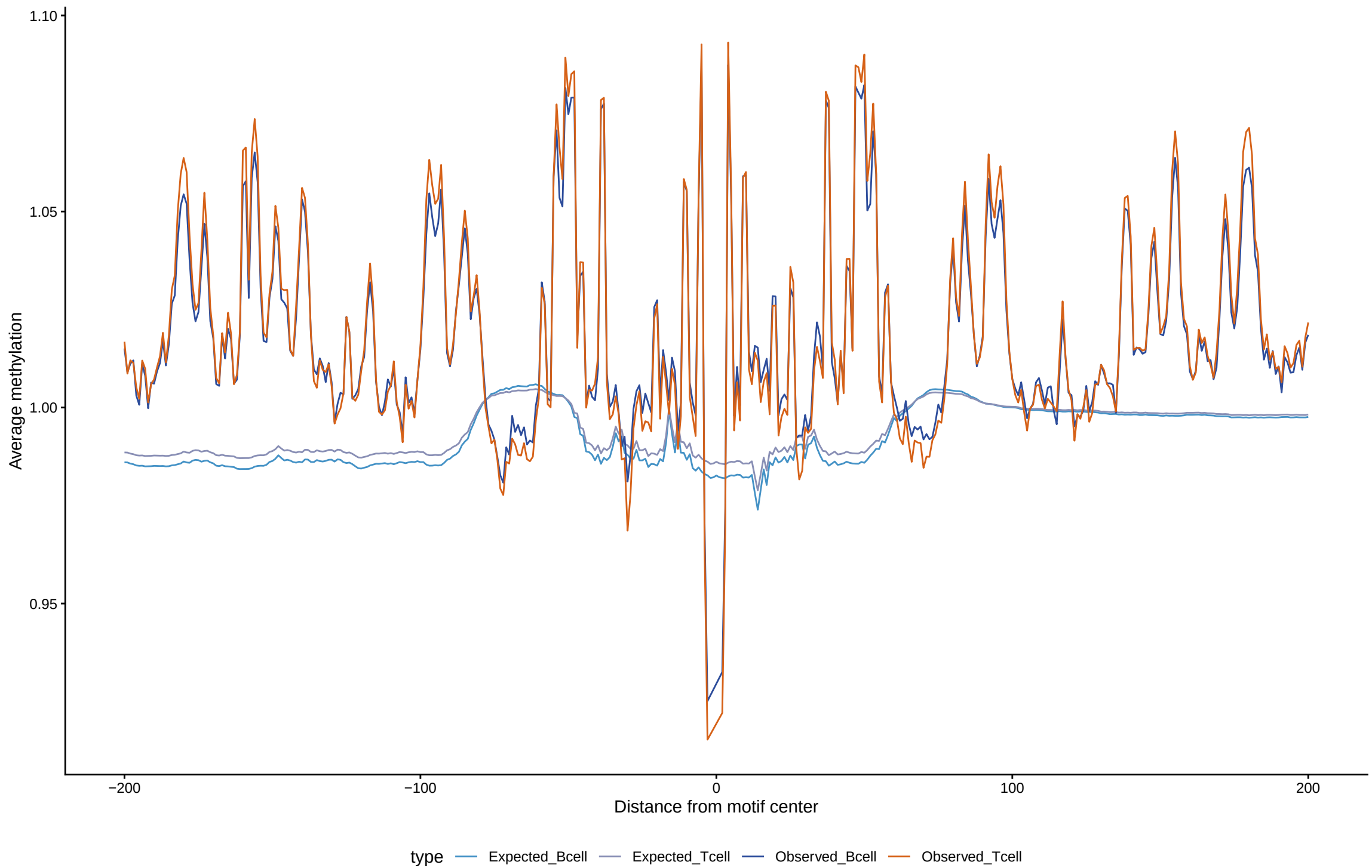
Expected vs observed footprints for ZNF354C
