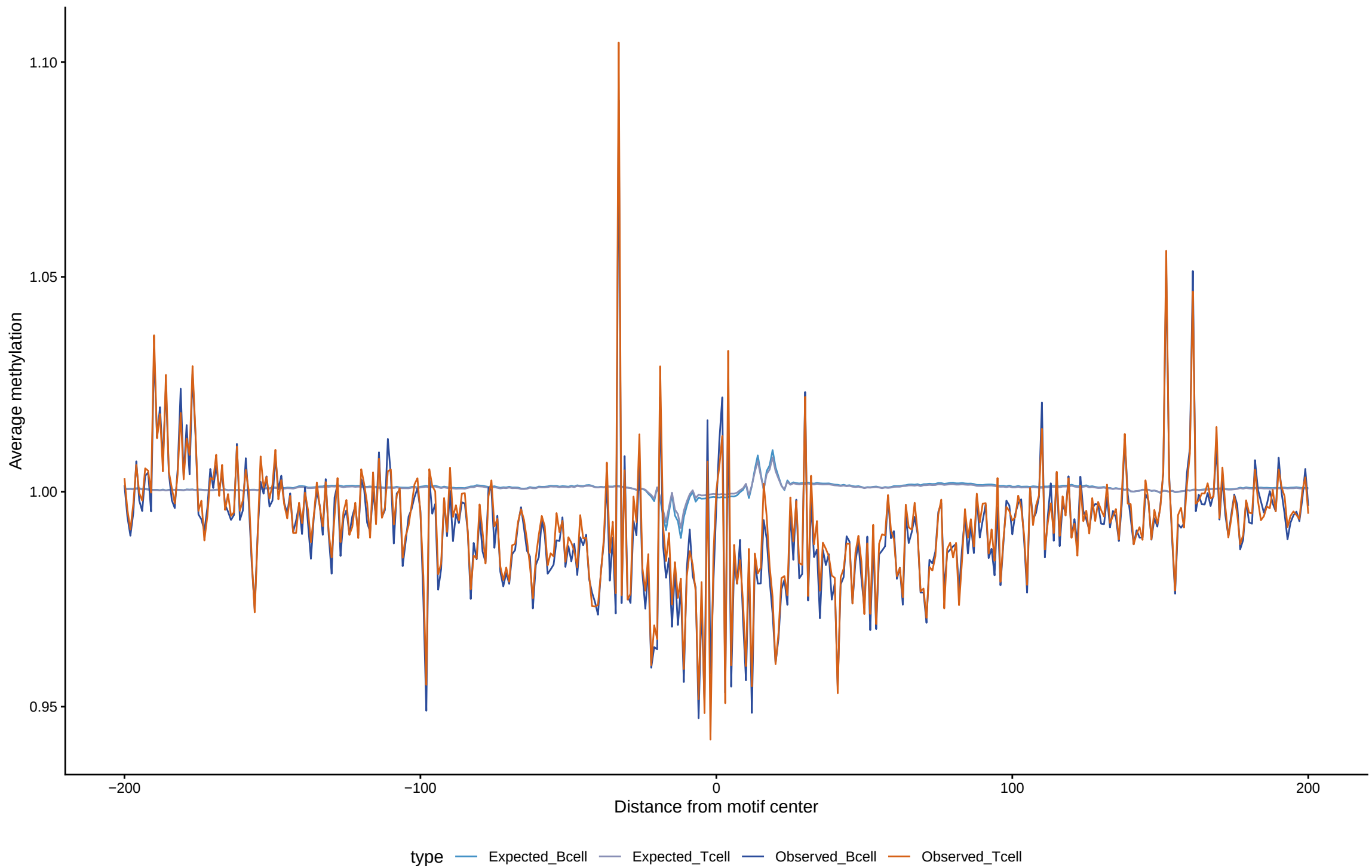
Expected vs observed footprints for ZNF528
