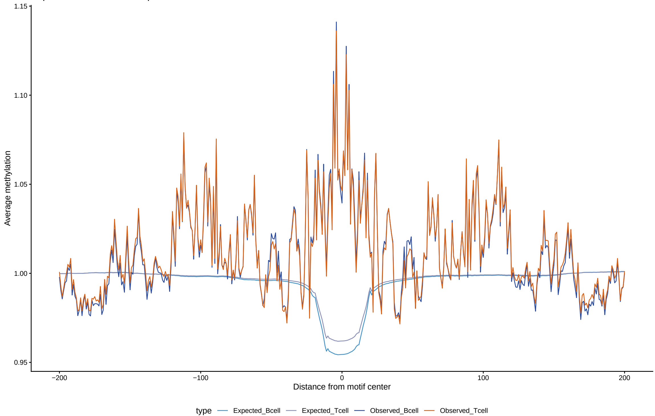
Expected vs observed footprints for ZNF740
