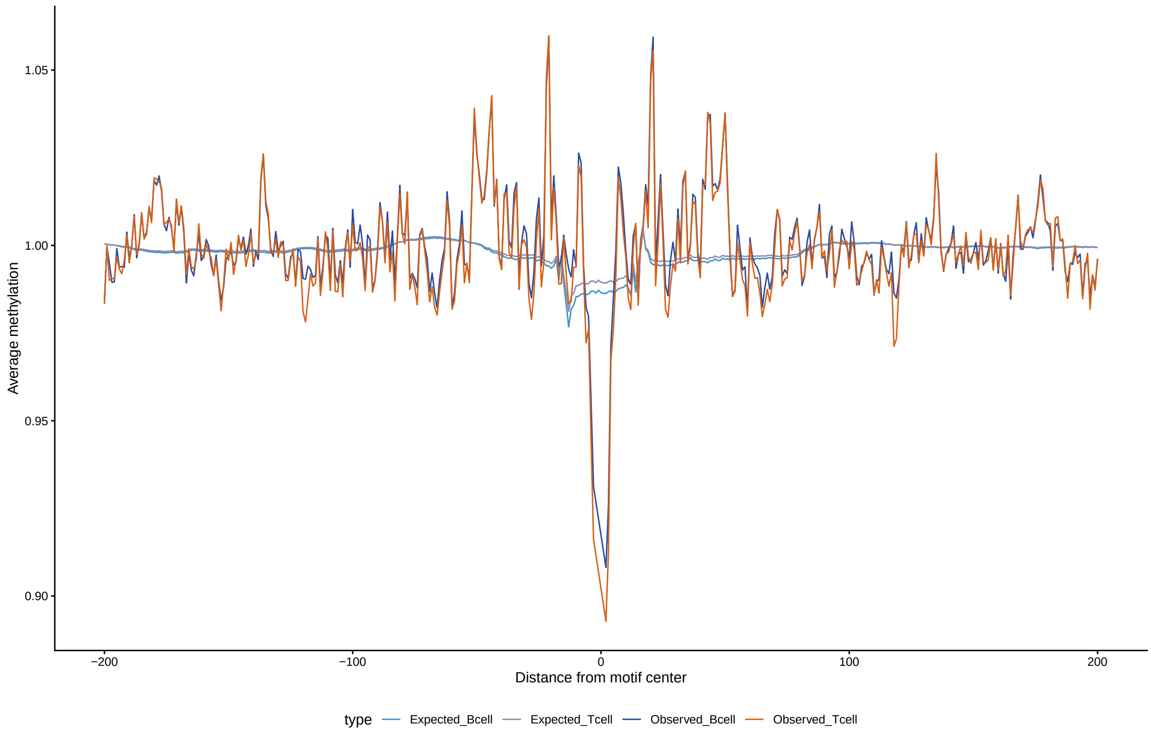
Expected vs observed footprints for ZNF75D
