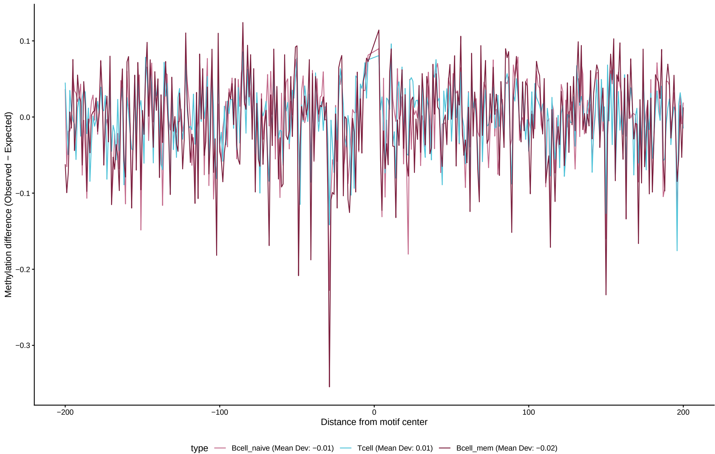
TF footprint difference for EMX1
