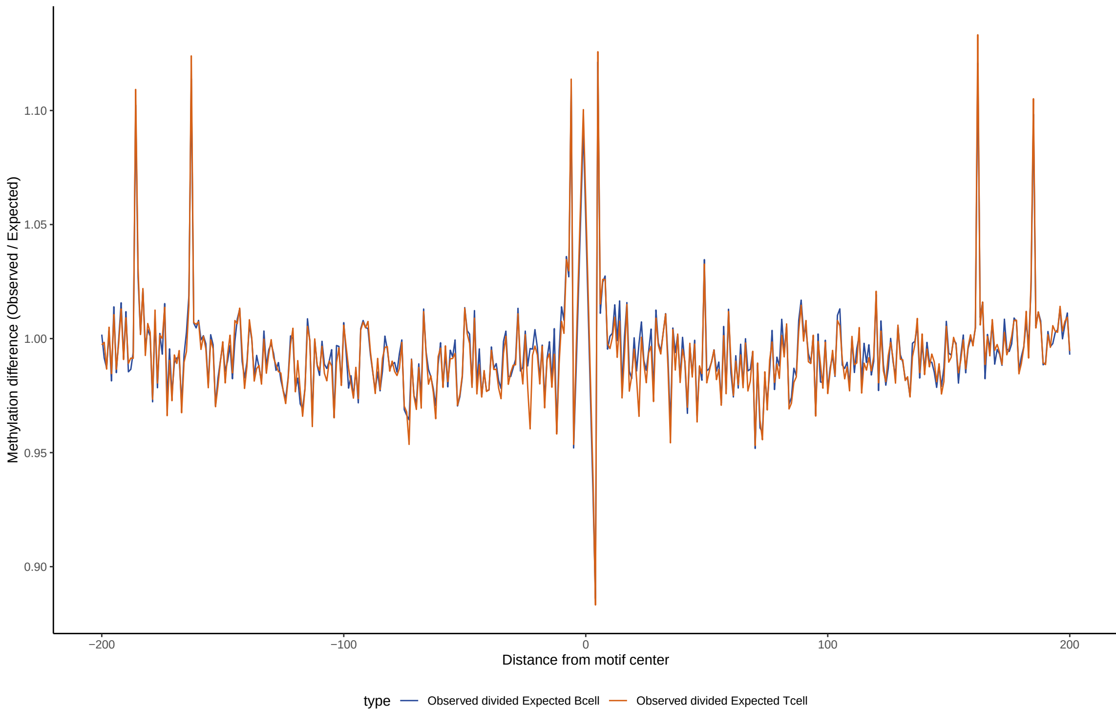
TF footprint difference for GCM1
