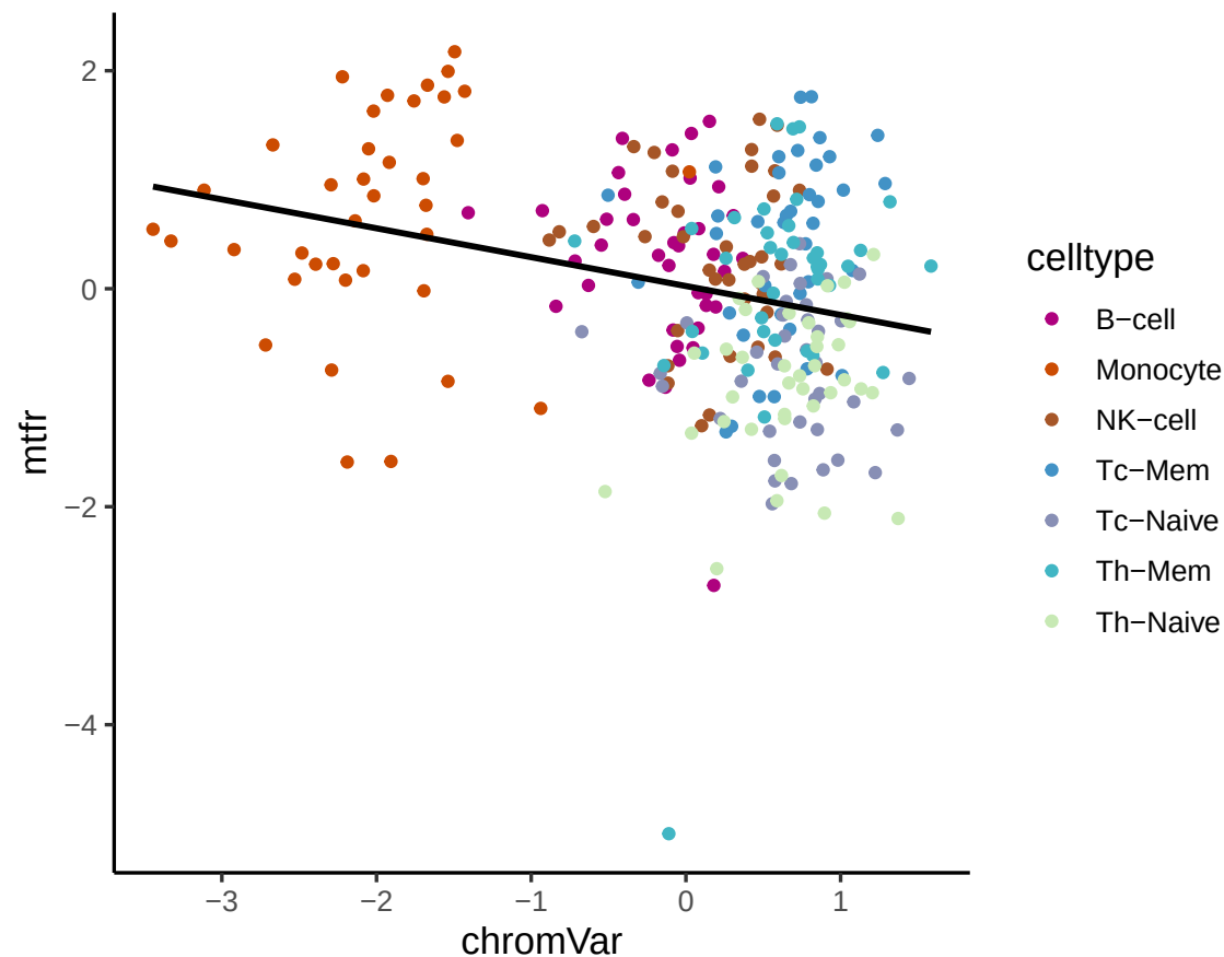
TF Activity Correlation (chromVar vs mtfr) for E2F2
