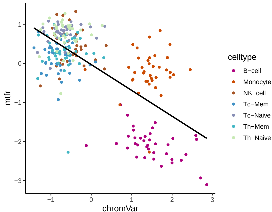
TF Activity Correlation (chromVar vs mtfr) for EBF3
