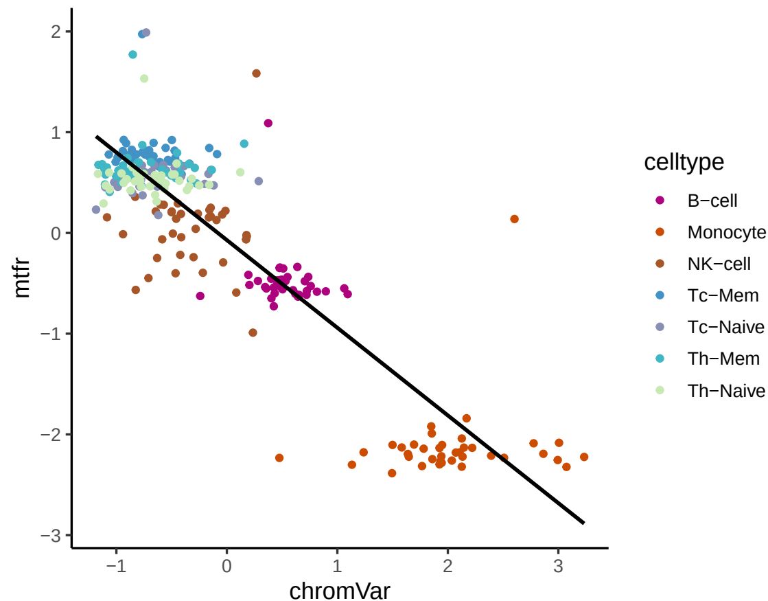
TF Activity Correlation (chromVar vs mtfr) for EHF
