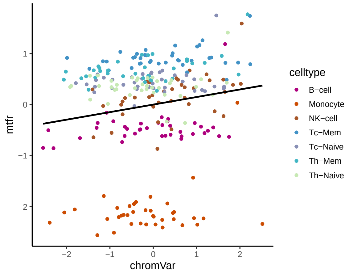
TF Activity Correlation (chromVar vs mtfr) for ELF4
