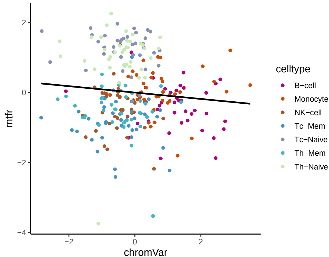
TF Activity Correlation (chromVar vs mtfr) for HEY2
