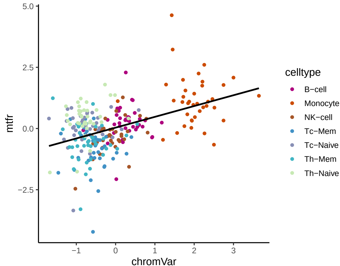
TF Activity Correlation (chromVar vs mtfr) for HIC2
